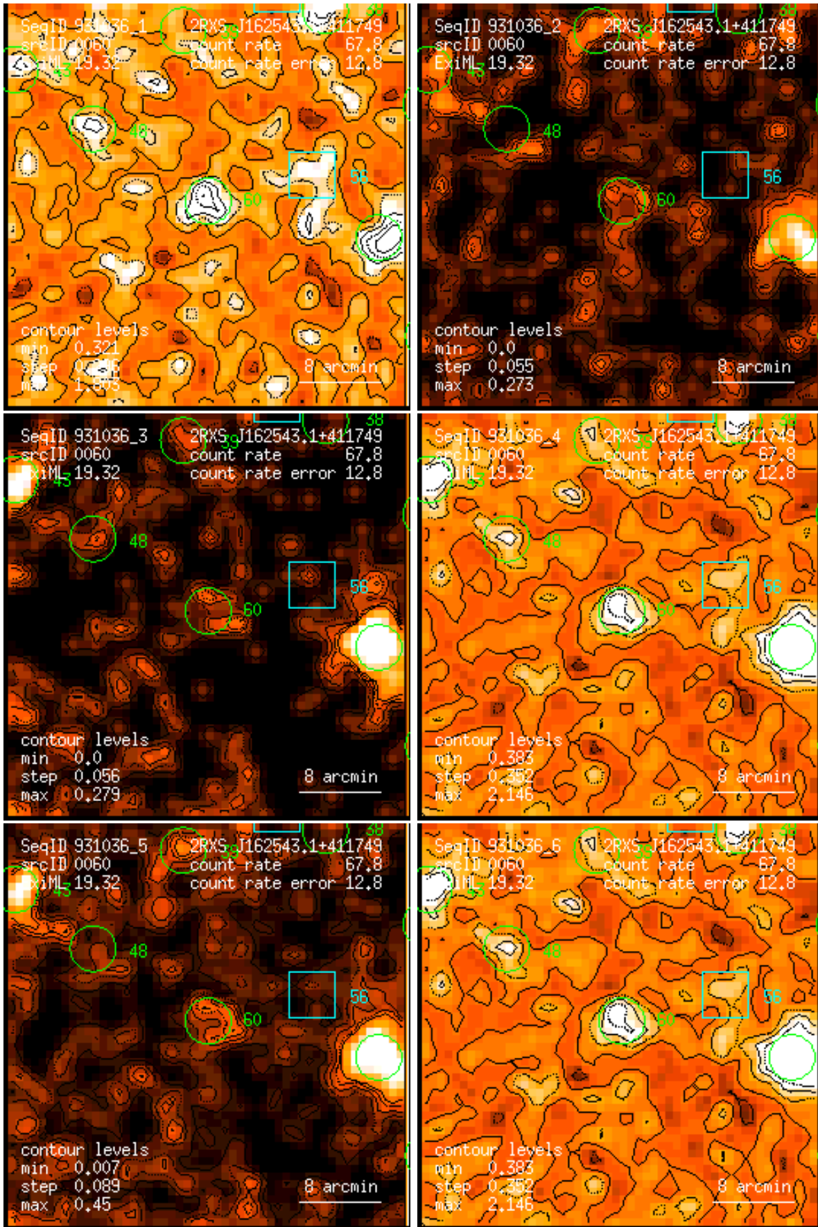
Figure 60: RASS 931036: detection 0060: band rate images, Gaussian filter: (1) PSPC channels 11 – 41, (2) 52 – 90, (3) 91 – 201, (4) 11 – 235, (5) 52 – 201, (6) 11 – 201. Broad band rates in counts/ks. Band rate contour levels in counts/ks/arcmin 2 .
