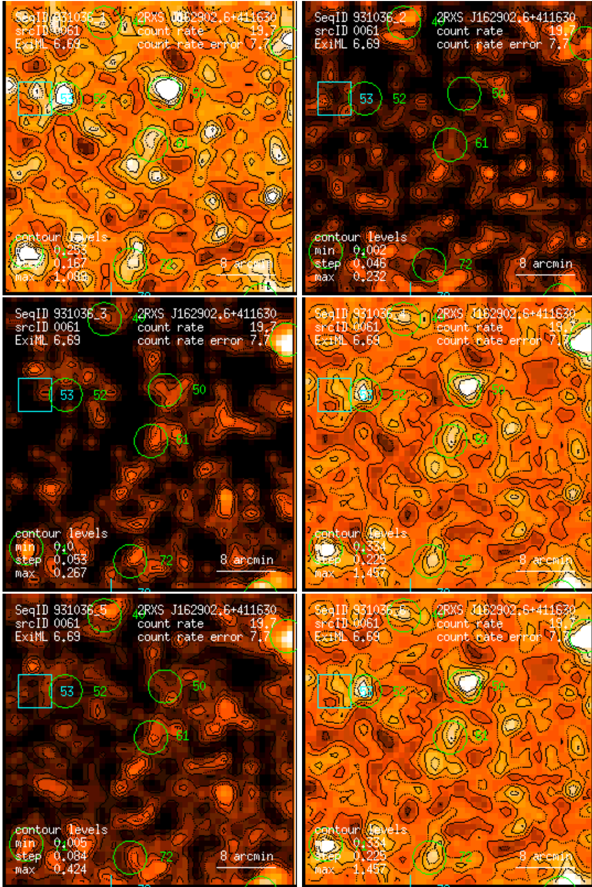
Figure 61: RASS 931036: detection 0061: band rate images, Gaussian filter: (1) PSPC channels 11 – 41, (2) 52 – 90, (3) 91 – 201, (4) 11 – 235, (5) 52 – 201, (6) 11 – 201. Broad band rates in counts/ks. Band rate contour levels in counts/ks/arcmin 2 .
