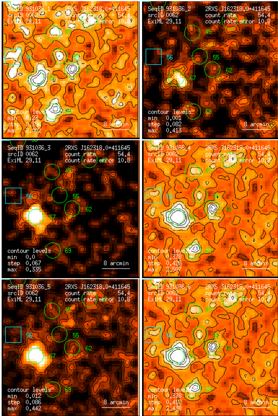
Figure 62: RASS 931036: detection 0062: band rate images, Gaussian filter: (1) PSPC channels 11 – 41, (2) 52 – 90, (3) 91 – 201, (4) 11 – 235, (5) 52 – 201, (6) 11 – 201. Broad band rates in counts/ks. Band rate contour levels in counts/ks/arcmin 2 .
