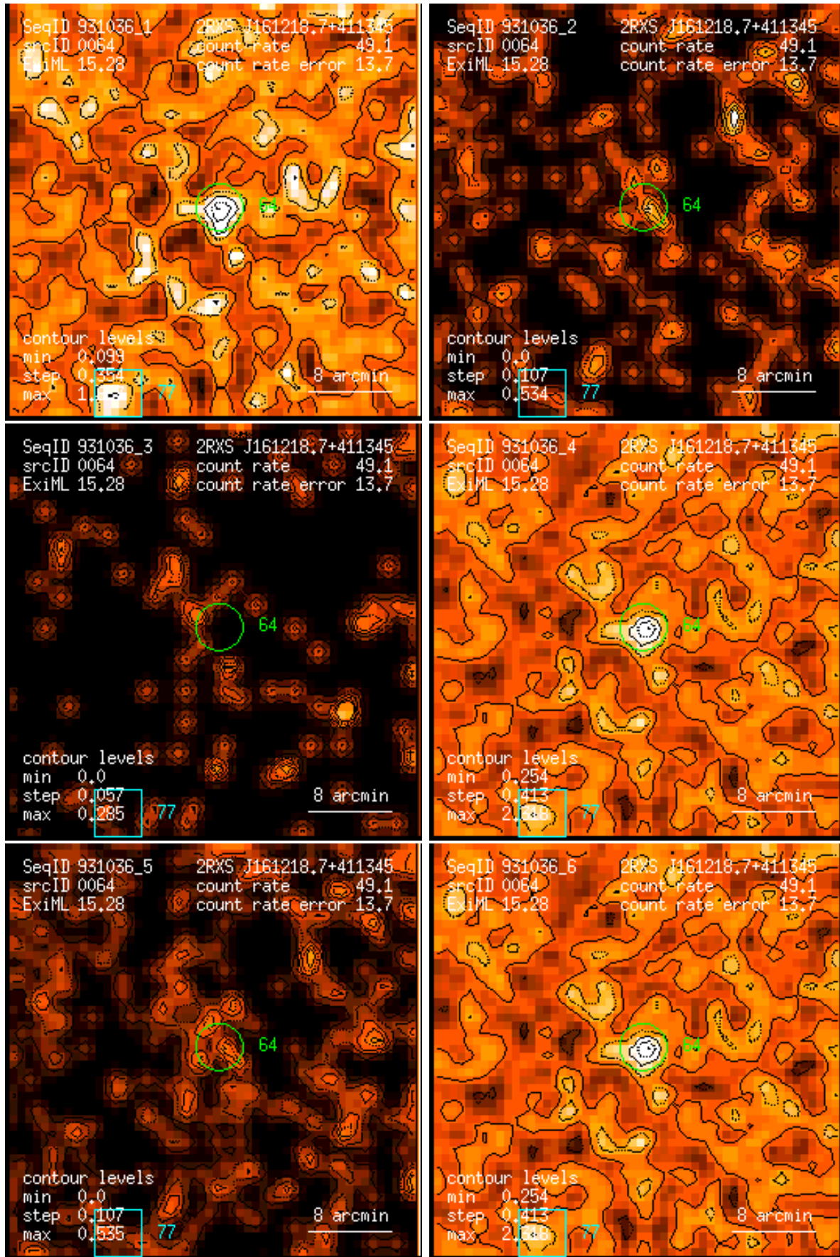
Figure 64: RASS 931036: detection 0064: band rate images, Gaussian filter: (1) PSPC channels 11 – 41, (2) 52 – 90, (3) 91 – 201, (4) 11 – 235, (5) 52 – 201, (6) 11 – 201. Broad band rates in counts/ks. Band rate contour levels in counts/ks/arcmin 2 .
