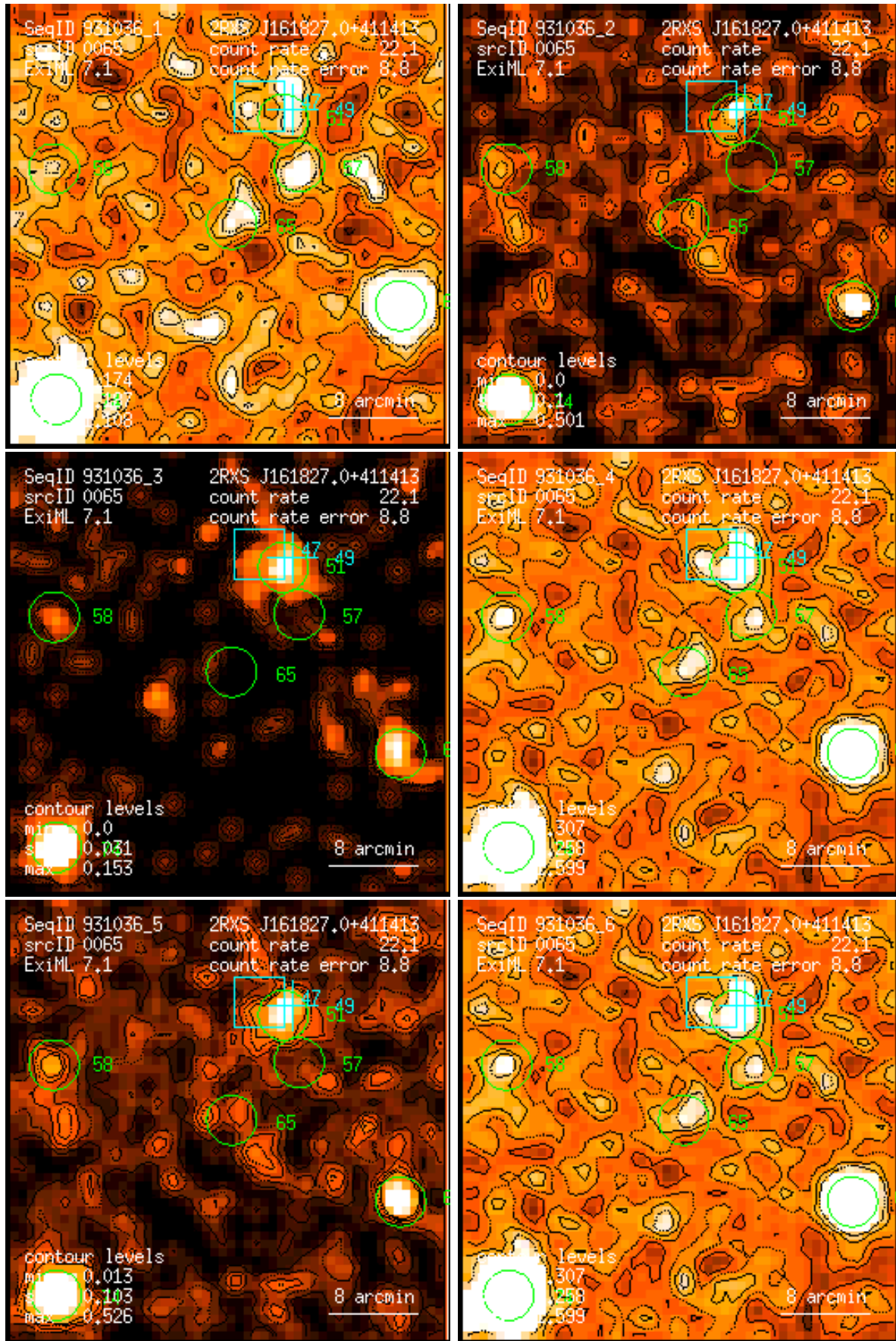
Figure 65: RASS 931036: detection 0065: band rate images, Gaussian filter: (1) PSPC channels 11 – 41, (2) 52 – 90, (3) 91 – 201, (4) 11 – 235, (5) 52 – 201, (6) 11 – 201. Broad band rates in counts/ks. Band rate contour levels in counts/ks/arcmin 2 .
