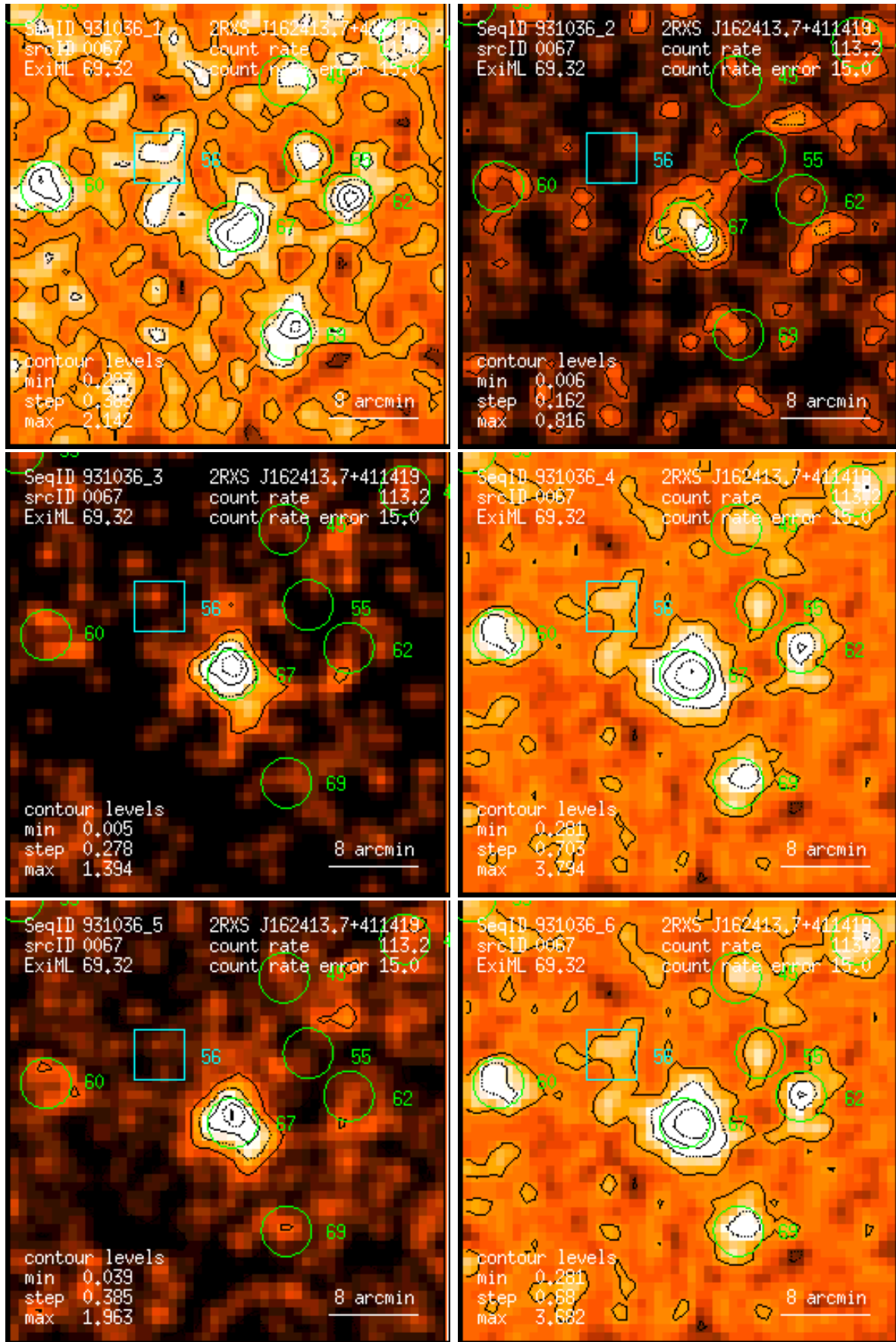
Figure 67: RASS 931036: detection 0067: band rate images, Gaussian filter: (1) PSPC channels 11 – 41, (2) 52 – 90, (3) 91 – 201, (4) 11 – 235, (5) 52 – 201, (6) 11 – 201. Broad band rates in counts/ks. Band rate contour levels in counts/ks/arcmin 2 .
