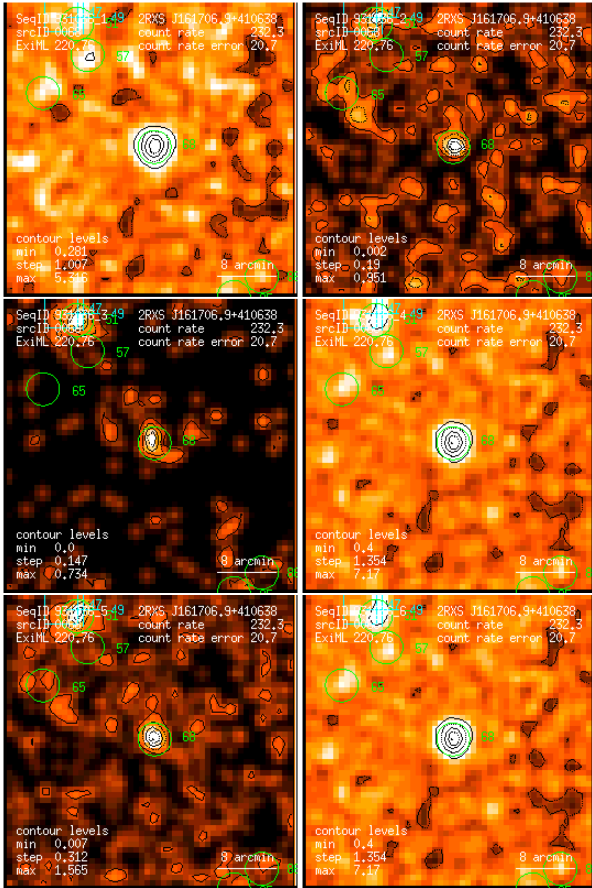
Figure 68: RASS 931036: detection 0068: band rate images, Gaussian filter: (1) PSPC channels 11 – 41, (2) 52 – 90, (3) 91 – 201, (4) 11 – 235, (5) 52 – 201, (6) 11 – 201. Broad band rates in counts/ks. Band rate contour levels in counts/ks/arcmin 2 .
