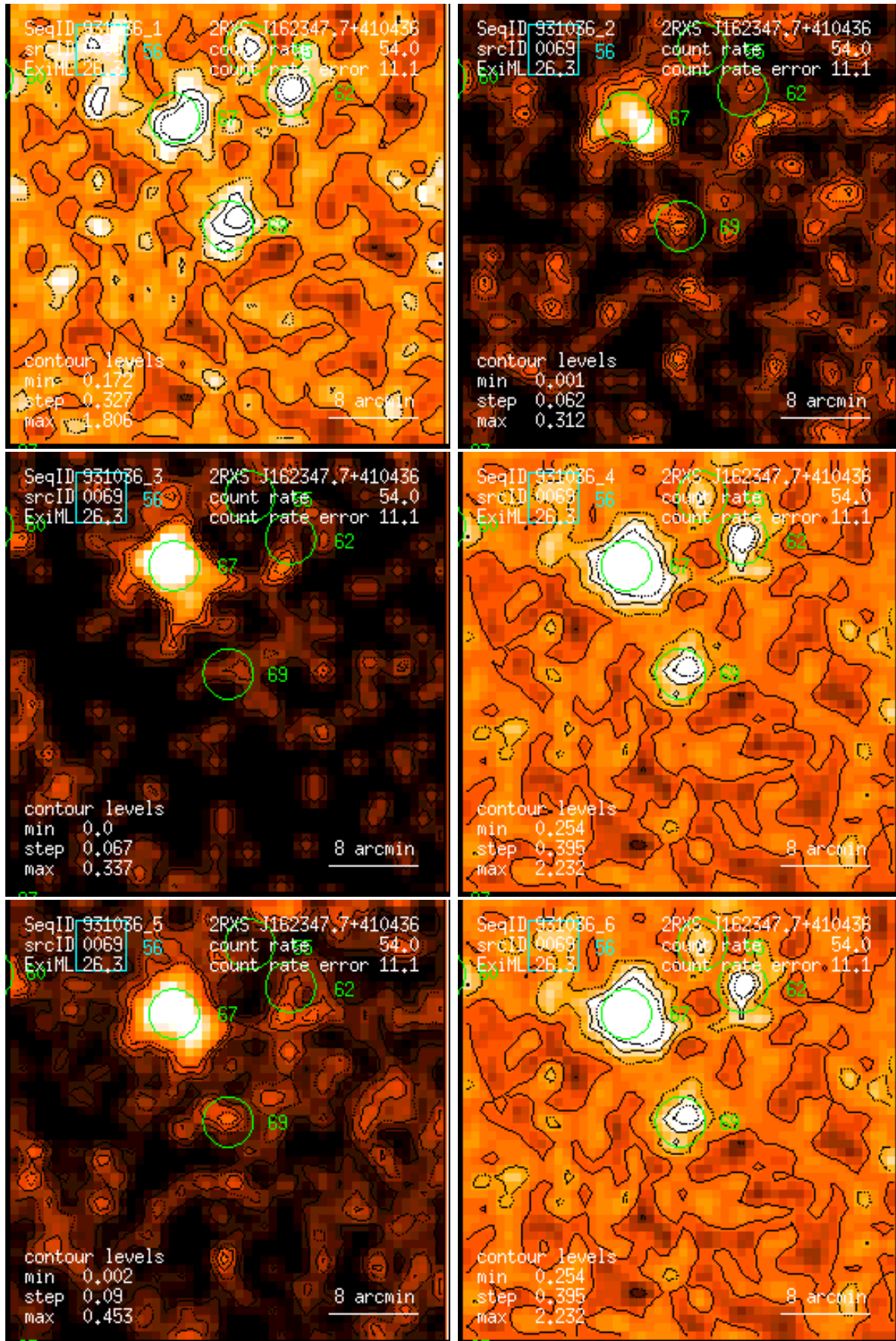
Figure 69: RASS 931036: detection 0069: band rate images, Gaussian filter: (1) PSPC channels 11 – 41, (2) 52 – 90, (3) 91 – 201, (4) 11 – 235, (5) 52 – 201, (6) 11 – 201. Broad band rates in counts/ks. Band rate contour levels in counts/ks/arcmin 2 .
