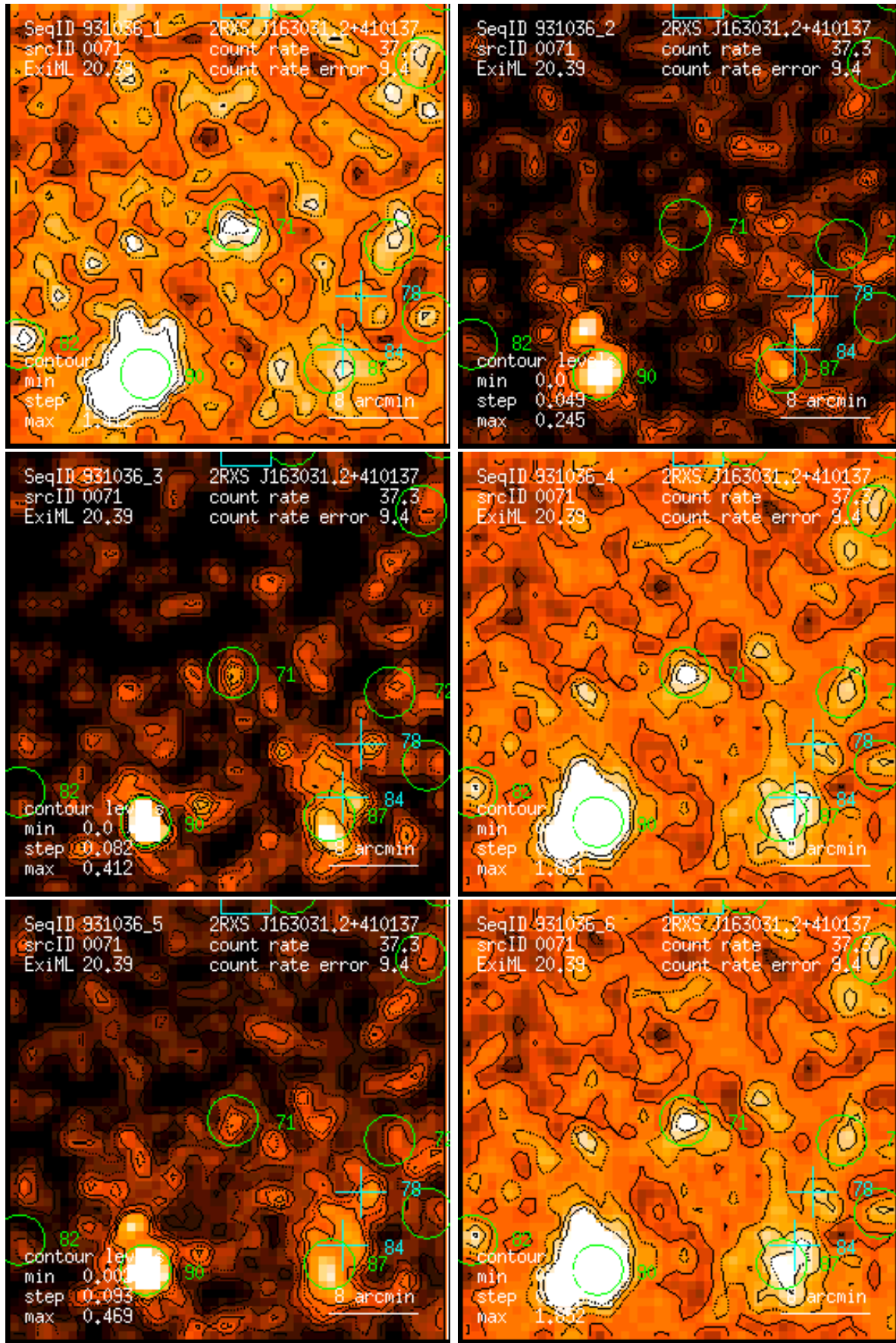
Figure 71: RASS 931036: detection 0071: band rate images, Gaussian filter: (1) PSPC channels 11 – 41, (2) 52 – 90, (3) 91 – 201, (4) 11 – 235, (5) 52 – 201, (6) 11 – 201. Broad band rates in counts/ks. Band rate contour levels in counts/ks/arcmin 2 .
