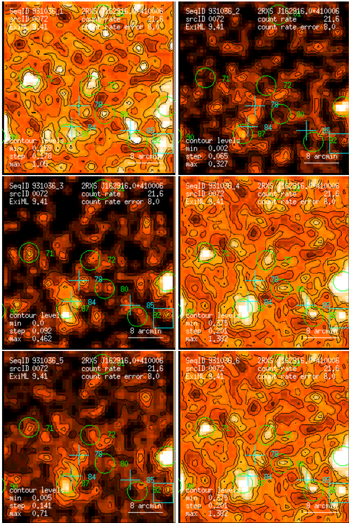
Figure 72: RASS 931036: detection 0072: band rate images, Gaussian filter: (1) PSPC channels 11 – 41, (2) 52 – 90, (3) 91 – 201, (4) 11 – 235, (5) 52 – 201, (6) 11 – 201. Broad band rates in counts/ks. Band rate contour levels in counts/ks/arcmin 2 .
