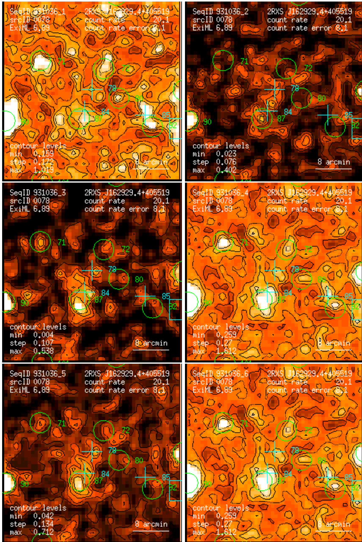
Figure 78: RASS 931036: detection 0078: band rate images, Gaussian filter: (1) PSPC channels 11 – 41, (2) 52 – 90, (3) 91 – 201, (4) 11 – 235, (5) 52 – 201, (6) 11 – 201. Broad band rates in counts/ks. Band rate contour levels in counts/ks/arcmin 2 .
