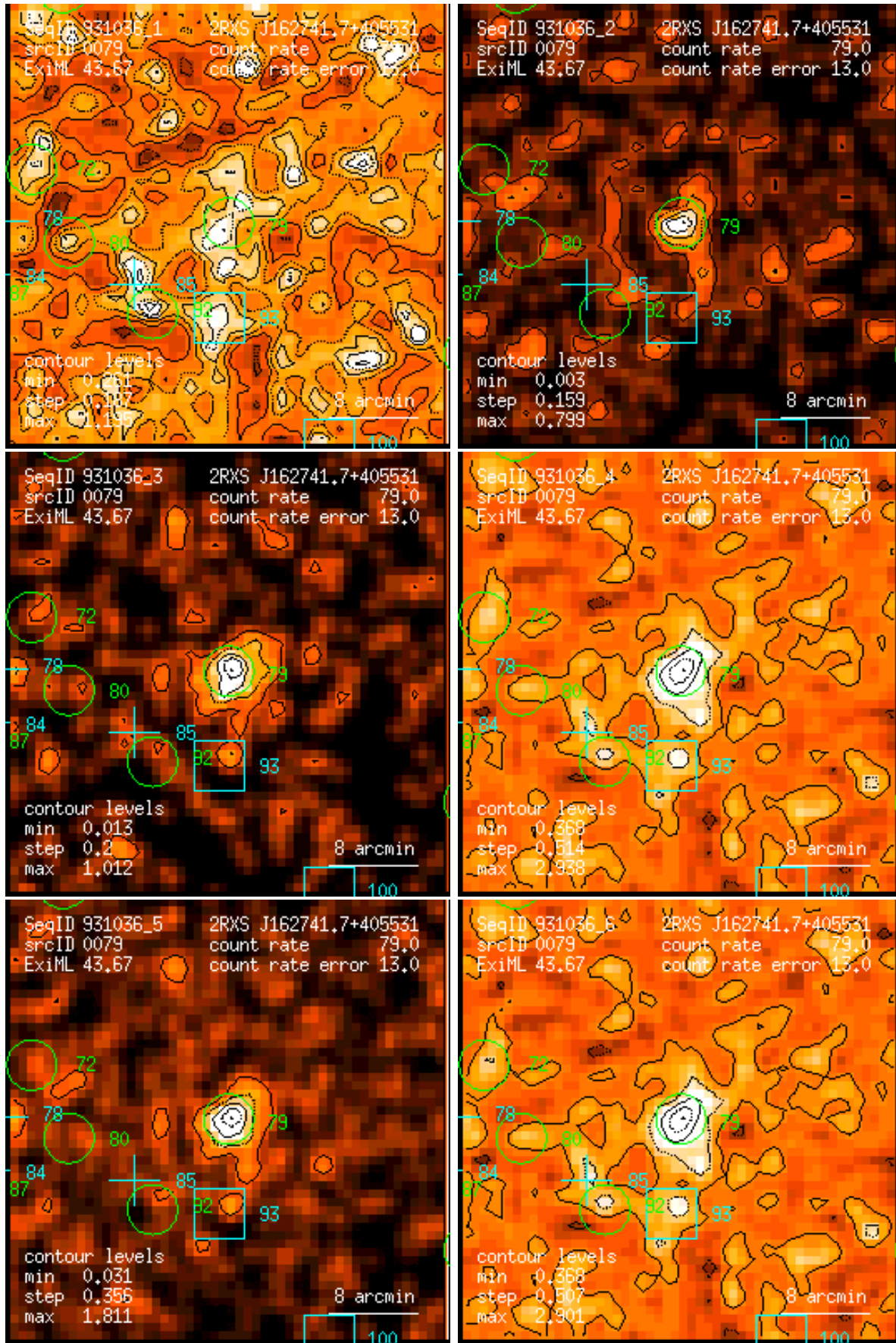
Figure 79: RASS 931036: detection 0079: band rate images, Gaussian filter: (1) PSPC channels 11 – 41, (2) 52 – 90, (3) 91 – 201, (4) 11 – 235, (5) 52 – 201, (6) 11 – 201. Broad band rates in counts/ks. Band rate contour levels in counts/ks/arcmin 2 .
