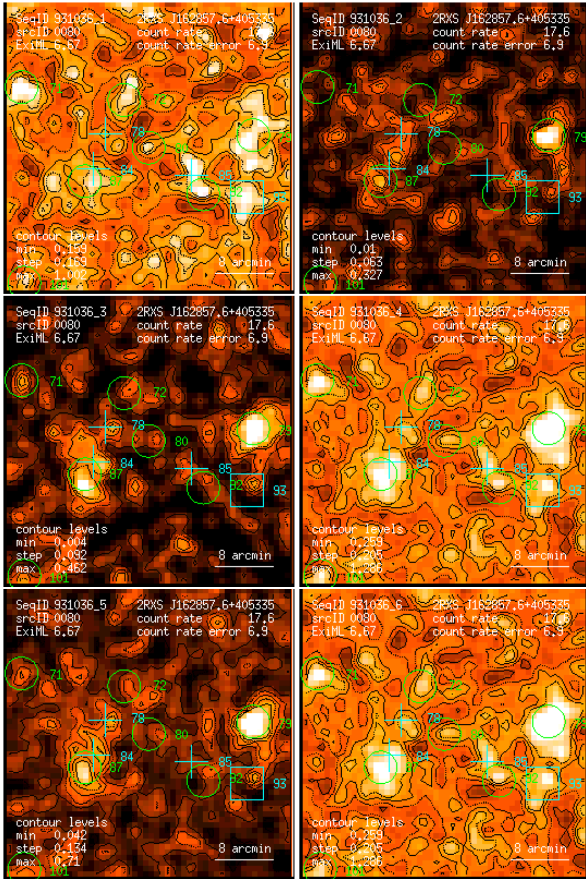
Figure 80: RASS 931036: detection 0080: band rate images, Gaussian filter: (1) PSPC channels 11 – 41, (2) 52 – 90, (3) 91 – 201, (4) 11 – 235, (5) 52 – 201, (6) 11 – 201. Broad band rates in counts/ks. Band rate contour levels in counts/ks/arcmin 2 .
