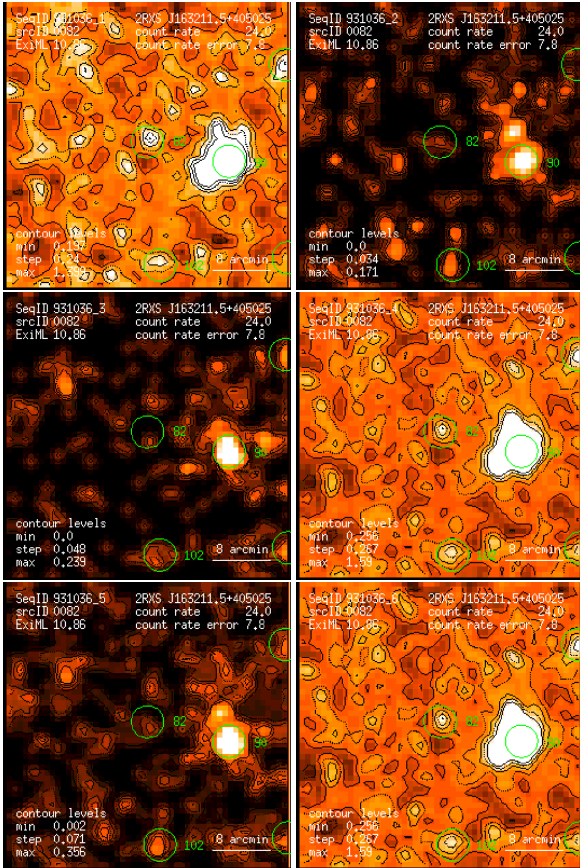
Figure 82: RASS 931036: detection 0082: band rate images, Gaussian filter: (1) PSPC channels 11 – 41, (2) 52 – 90, (3) 91 – 201, (4) 11 – 235, (5) 52 – 201, (6) 11 – 201. Broad band rates in counts/ks. Band rate contour levels in counts/ks/arcmin 2 .
