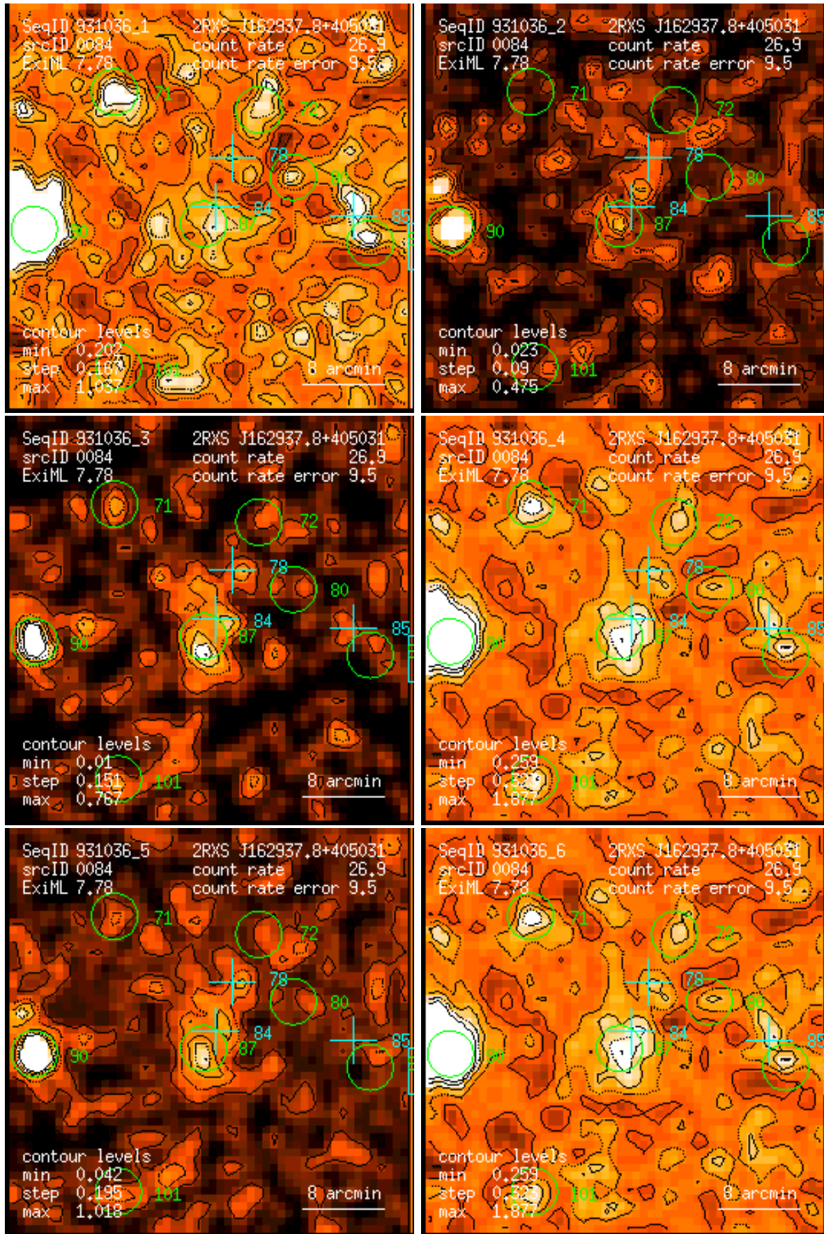
Figure 84: RASS 931036: detection 0084: band rate images, Gaussian filter: (1) PSPC channels 11 – 41, (2) 52 – 90, (3) 91 – 201, (4) 11 – 235, (5) 52 – 201, (6) 11 – 201. Broad band rates in counts/ks. Band rate contour levels in counts/ks/arcmin 2 .
