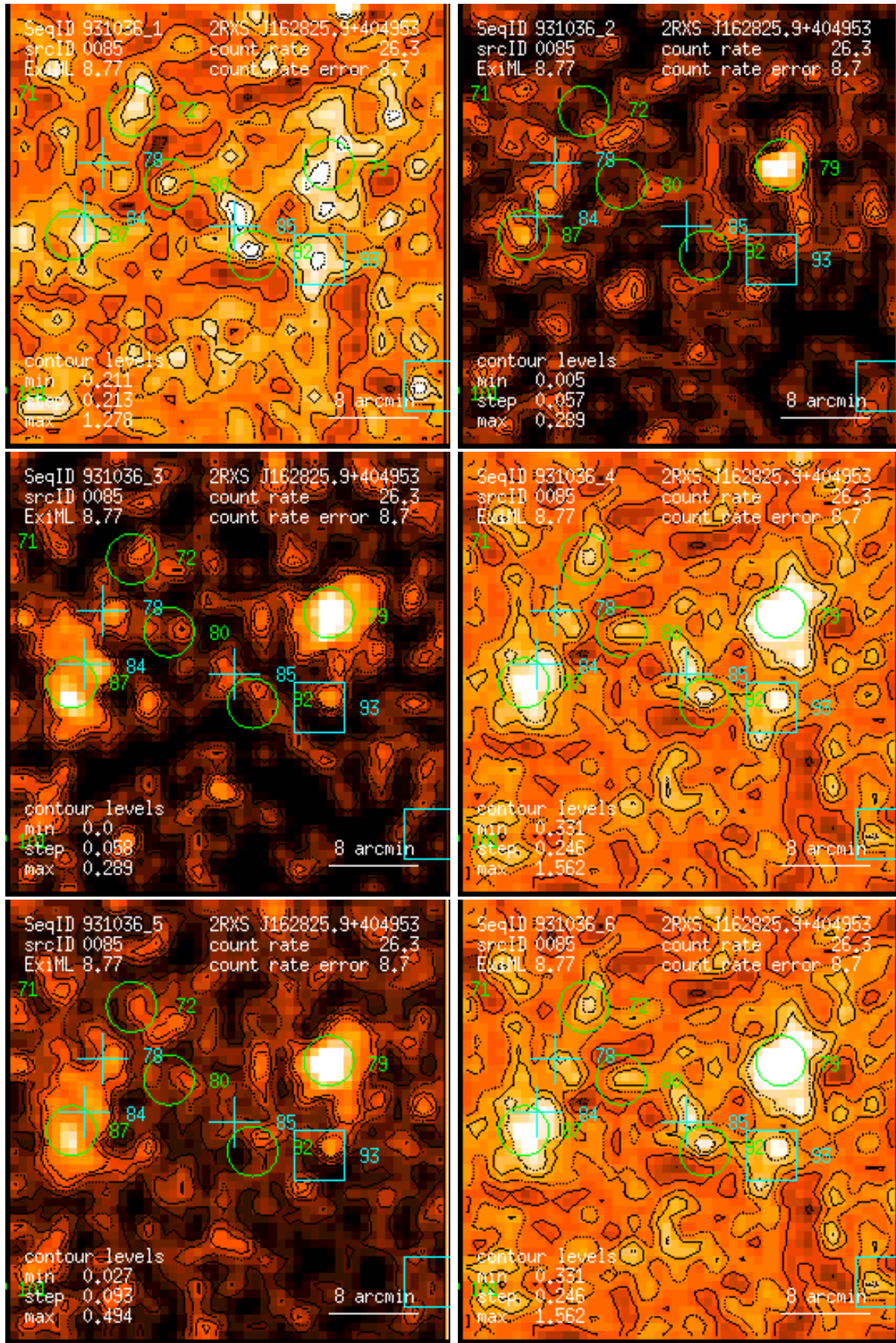
Figure 85: RASS 931036: detection 0085: band rate images, Gaussian filter: (1) PSPC channels 11 – 41, (2) 52 – 90, (3) 91 – 201, (4) 11 – 235, (5) 52 – 201, (6) 11 – 201. Broad band rates in counts/ks. Band rate contour levels in counts/ks/arcmin 2 .
