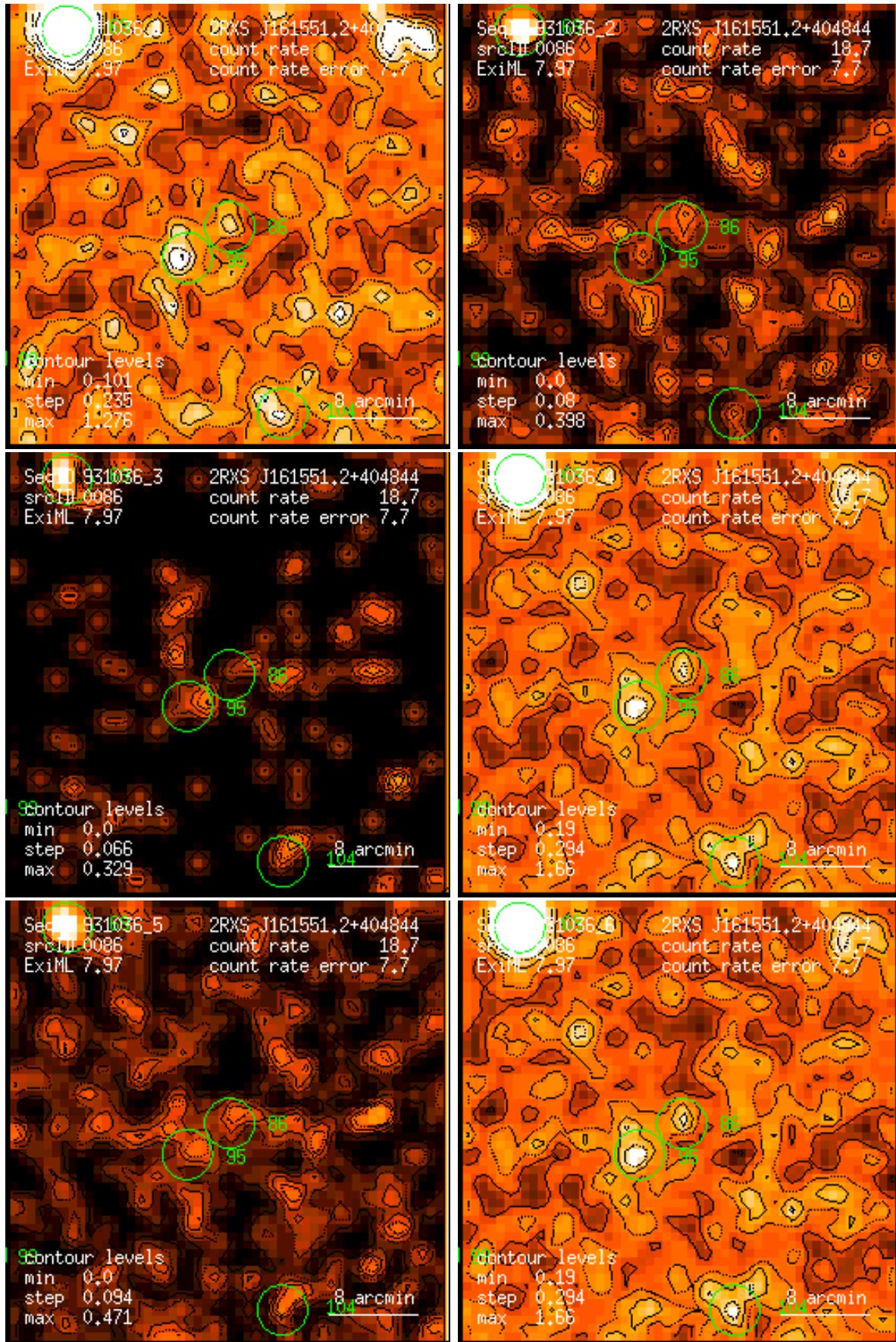
Figure 86: RASS 931036: detection 0086: band rate images, Gaussian filter: (1) PSPC channels 11 – 41, (2) 52 – 90, (3) 91 – 201, (4) 11 – 235, (5) 52 – 201, (6) 11 – 201. Broad band rates in counts/ks. Band rate contour levels in counts/ks/arcmin 2 .
