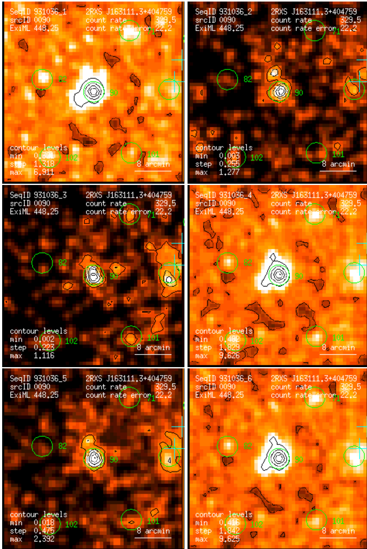
Figure 90: RASS 931036: detection 0090: band rate images, Gaussian filter: (1) PSPC channels 11 – 41, (2) 52 – 90, (3) 91 – 201, (4) 11 – 235, (5) 52 – 201, (6) 11 – 201. Broad band rates in counts/ks. Band rate contour levels in counts/ks/arcmin 2 .
