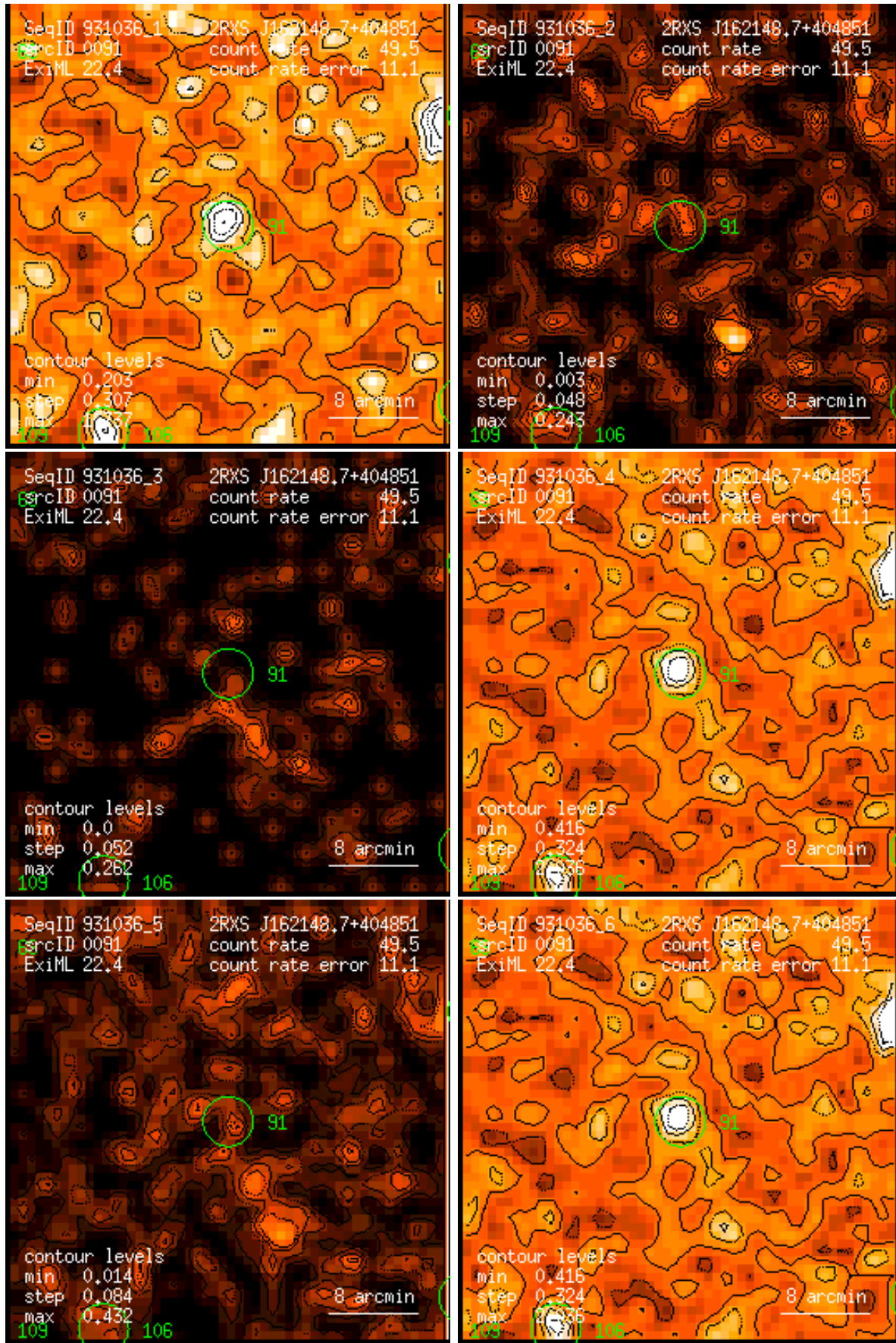
Figure 91: RASS 931036: detection 0091: band rate images, Gaussian filter: (1) PSPC channels 11 – 41, (2) 52 – 90, (3) 91 – 201, (4) 11 – 235, (5) 52 – 201, (6) 11 – 201. Broad band rates in counts/ks. Band rate contour levels in counts/ks/arcmin 2 .
