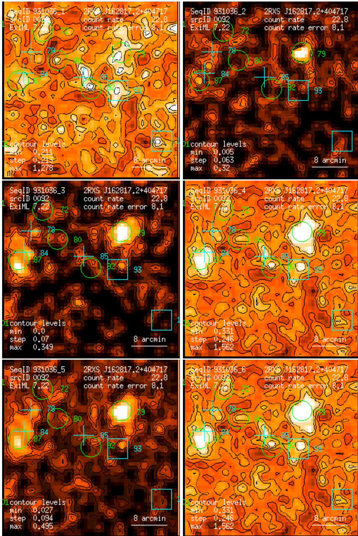
Figure 92: RASS 931036: detection 0092: band rate images, Gaussian filter: (1) PSPC channels 11 – 41, (2) 52 – 90, (3) 91 – 201, (4) 11 – 235, (5) 52 – 201, (6) 11 – 201. Broad band rates in counts/ks. Band rate contour levels in counts/ks/arcmin 2 .
