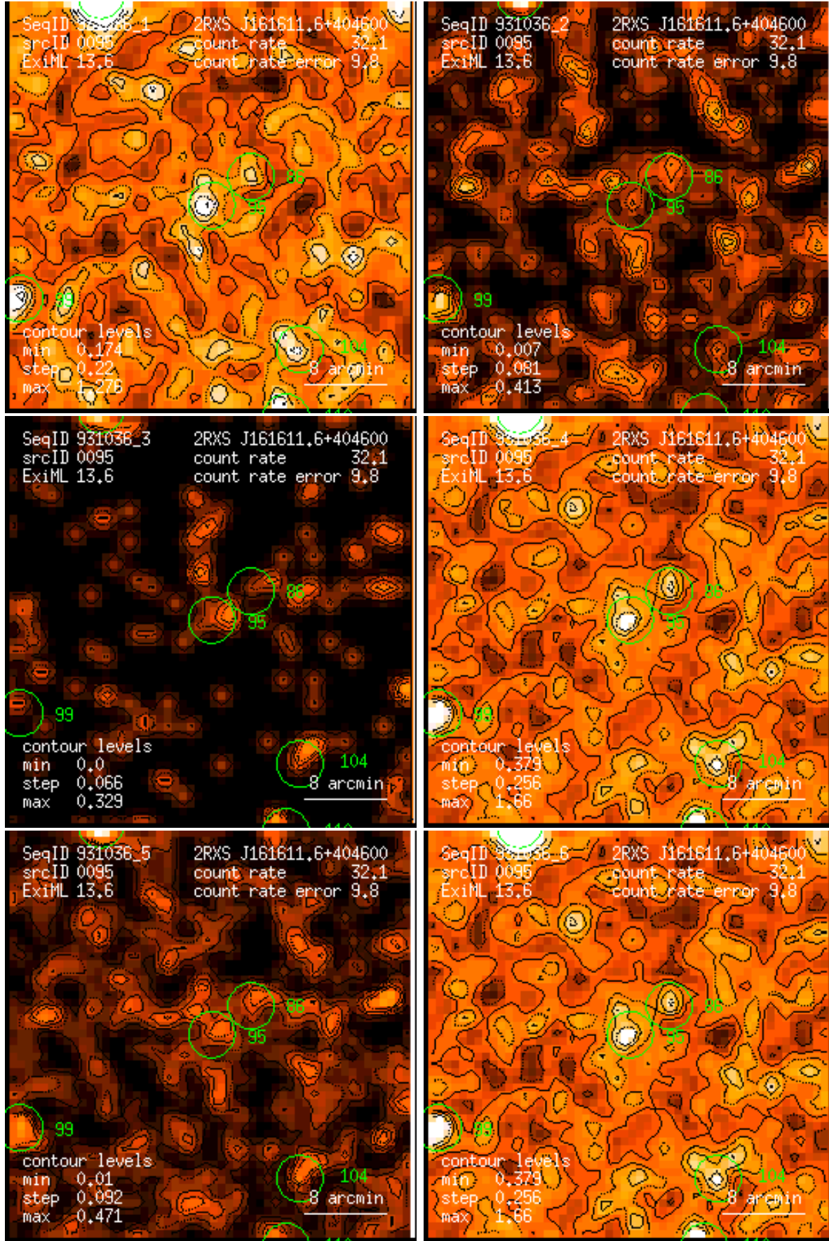
Figure 95: RASS 931036: detection 0095: band rate images, Gaussian filter: (1) PSPC channels 11 – 41, (2) 52 – 90, (3) 91 – 201, (4) 11 – 235, (5) 52 – 201, (6) 11 – 201. Broad band rates in counts/ks. Band rate contour levels in counts/ks/arcmin 2 .
