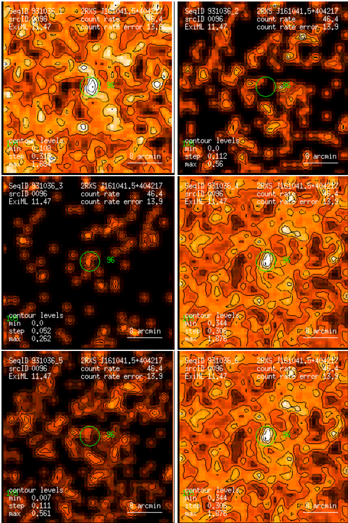
Figure 96: RASS 931036: detection 0096: band rate images, Gaussian filter: (1) PSPC channels 11 – 41, (2) 52 – 90, (3) 91 – 201, (4) 11 – 235, (5) 52 – 201, (6) 11 – 201. Broad band rates in counts/ks. Band rate contour levels in counts/ks/arcmin 2 .
