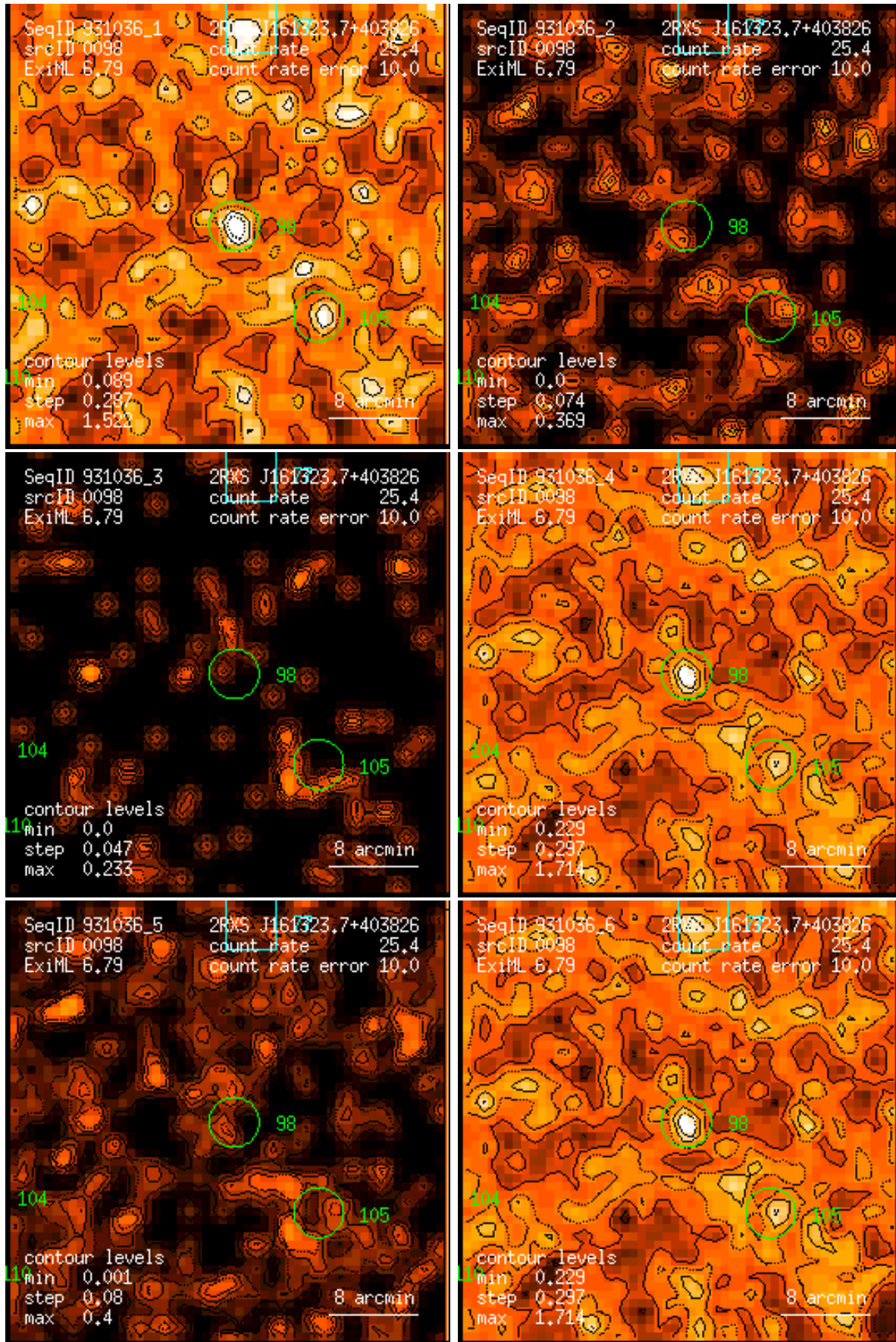
Figure 98: RASS 931036: detection 0098: band rate images, Gaussian filter: (1) PSPC channels 11 – 41, (2) 52 – 90, (3) 91 – 201, (4) 11 – 235, (5) 52 – 201, (6) 11 – 201. Broad band rates in counts/ks. Band rate contour levels in counts/ks/arcmin 2 .
