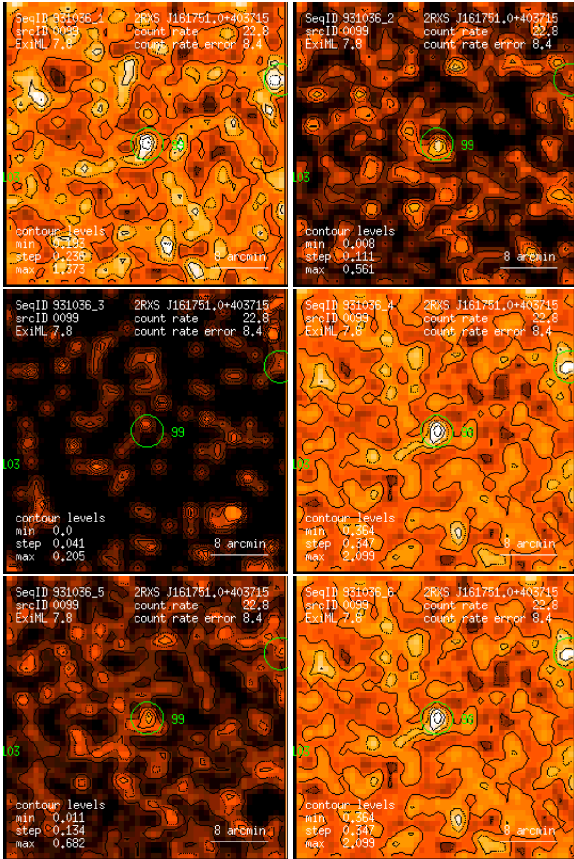
Figure 99: RASS 931036: detection 0099: band rate images, Gaussian filter: (1) PSPC channels 11 – 41, (2) 52 – 90, (3) 91 – 201, (4) 11 – 235, (5) 52 – 201, (6) 11 – 201. Broad band rates in counts/ks. Band rate contour levels in counts/ks/arcmin 2 .
