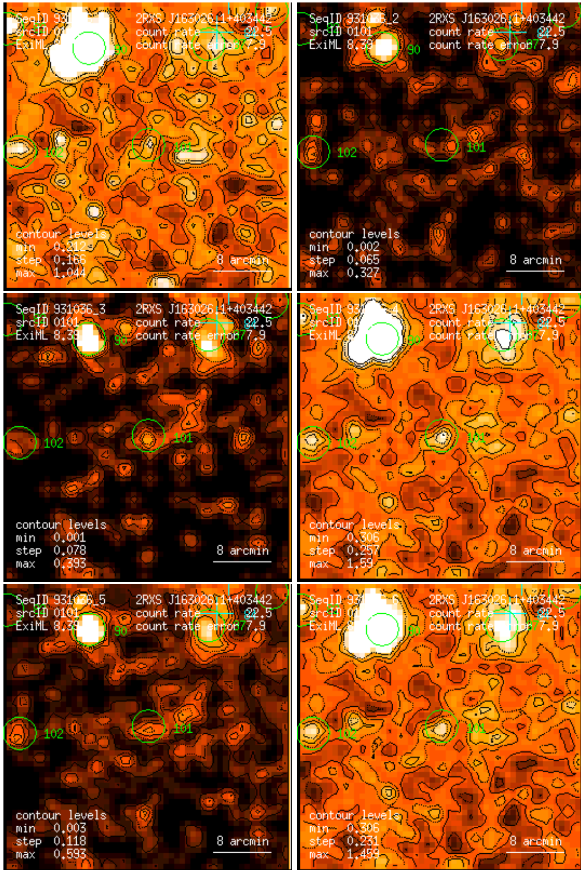
Figure 101: RASS 931036: detection 0101: band rate images, Gaussian filter: (1) PSPC channels 11 – 41, (2) 52 – 90, (3) 91 – 201, (4) 11 – 235, (5) 52 – 201, (6) 11 – 201. Broad band rates in counts/ks. Band rate contour levels in counts/ks/arcmin 2 .
