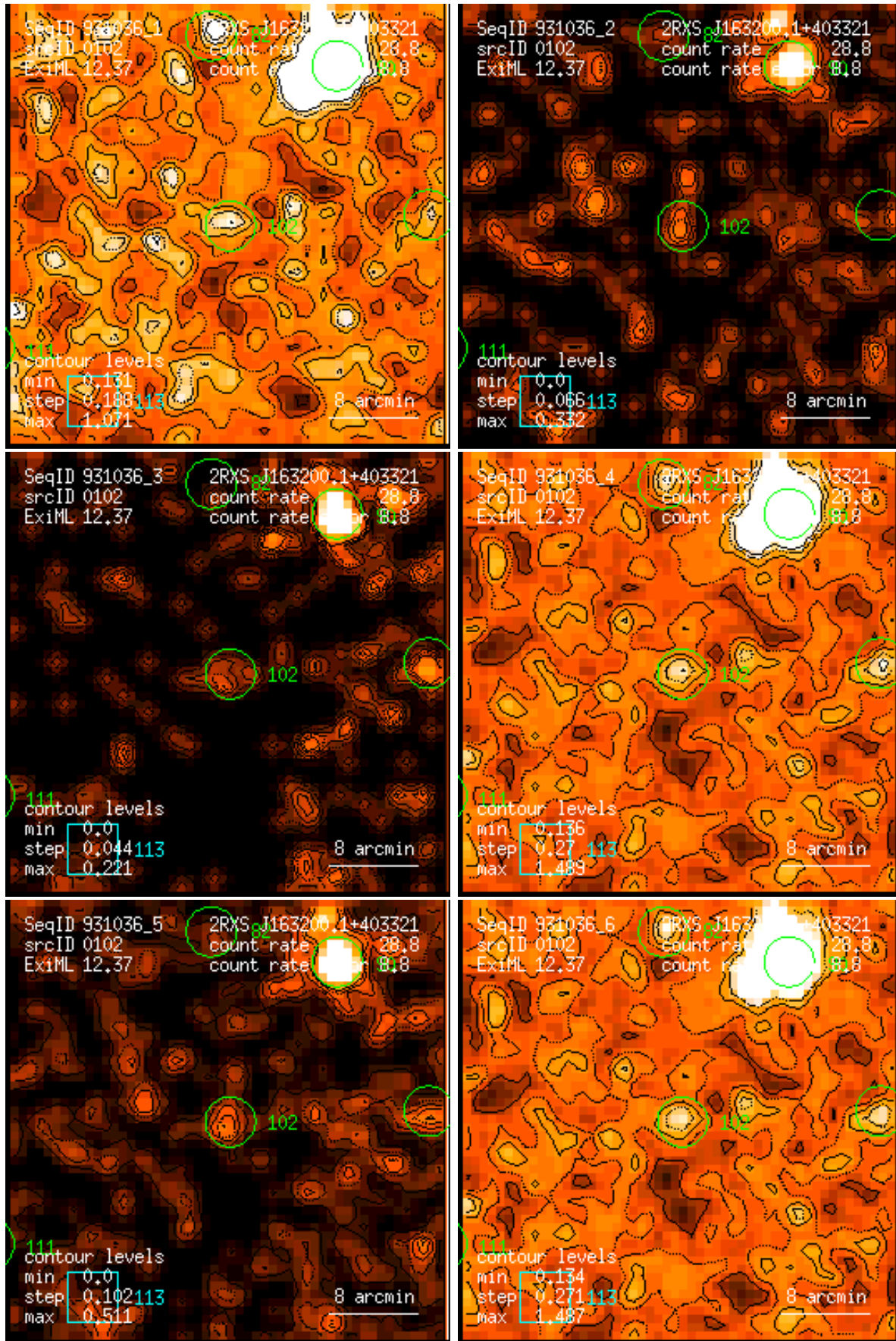
Figure 102: RASS 931036: detection 0102: band rate images, Gaussian filter: (1) PSPC channels 11 – 41, (2) 52 – 90, (3) 91 – 201, (4) 11 – 235, (5) 52 – 201, (6) 11 – 201. Broad band rates in counts/ks. Band rate contour levels in counts/ks/arcmin 2 .
