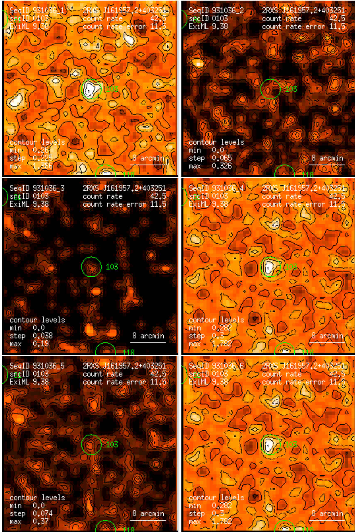
Figure 103: RASS 931036: detection 0103: band rate images, Gaussian filter: (1) PSPC channels 11 – 41, (2) 52 – 90, (3) 91 – 201, (4) 11 – 235, (5) 52 – 201, (6) 11 – 201. Broad band rates in counts/ks. Band rate contour levels in counts/ks/arcmin 2 .
