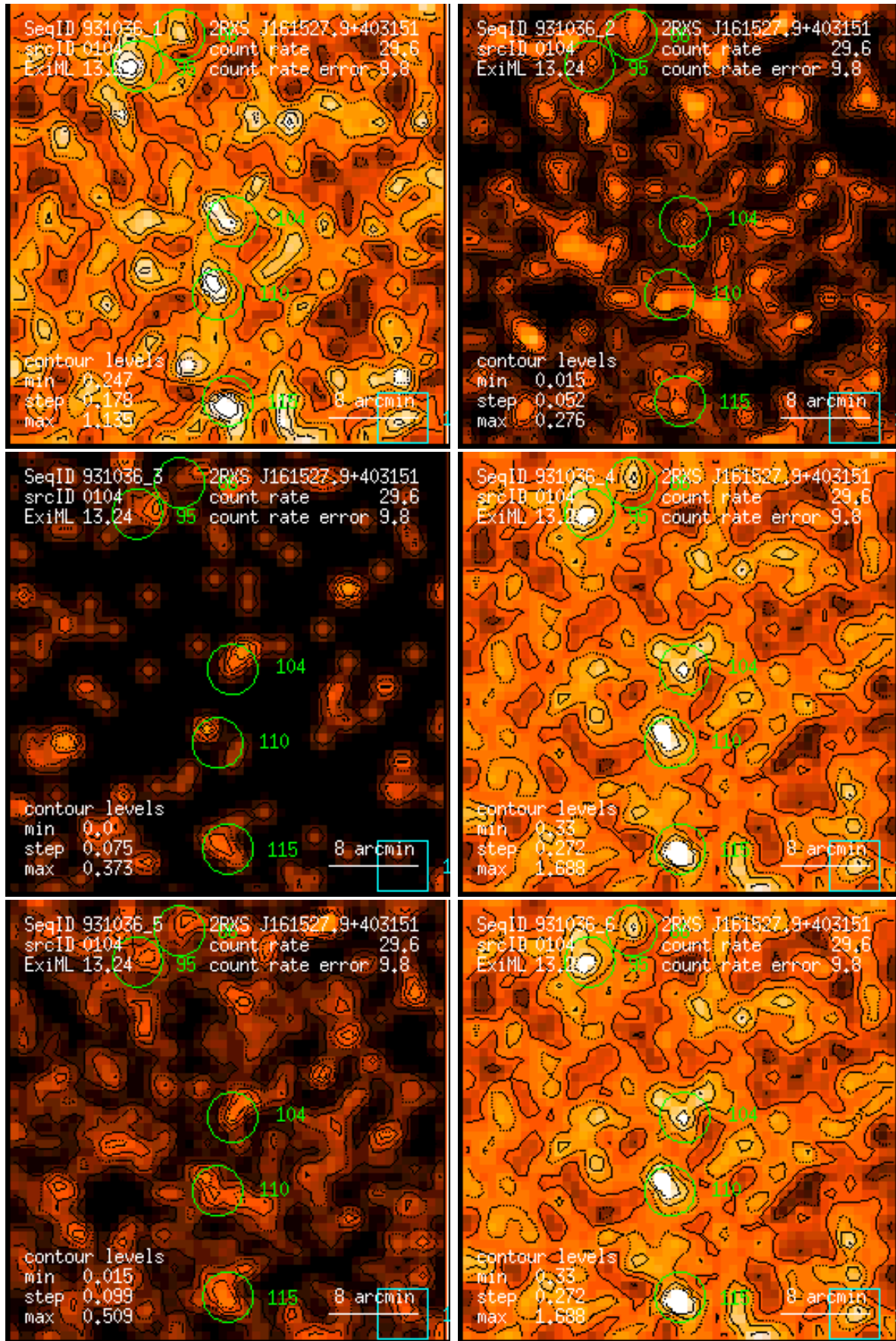
Figure 104: RASS 931036: detection 0104: band rate images, Gaussian filter: (1) PSPC channels 11 – 41, (2) 52 – 90, (3) 91 – 201, (4) 11 – 235, (5) 52 – 201, (6) 11 – 201. Broad band rates in counts/ks. Band rate contour levels in counts/ks/arcmin 2 .
