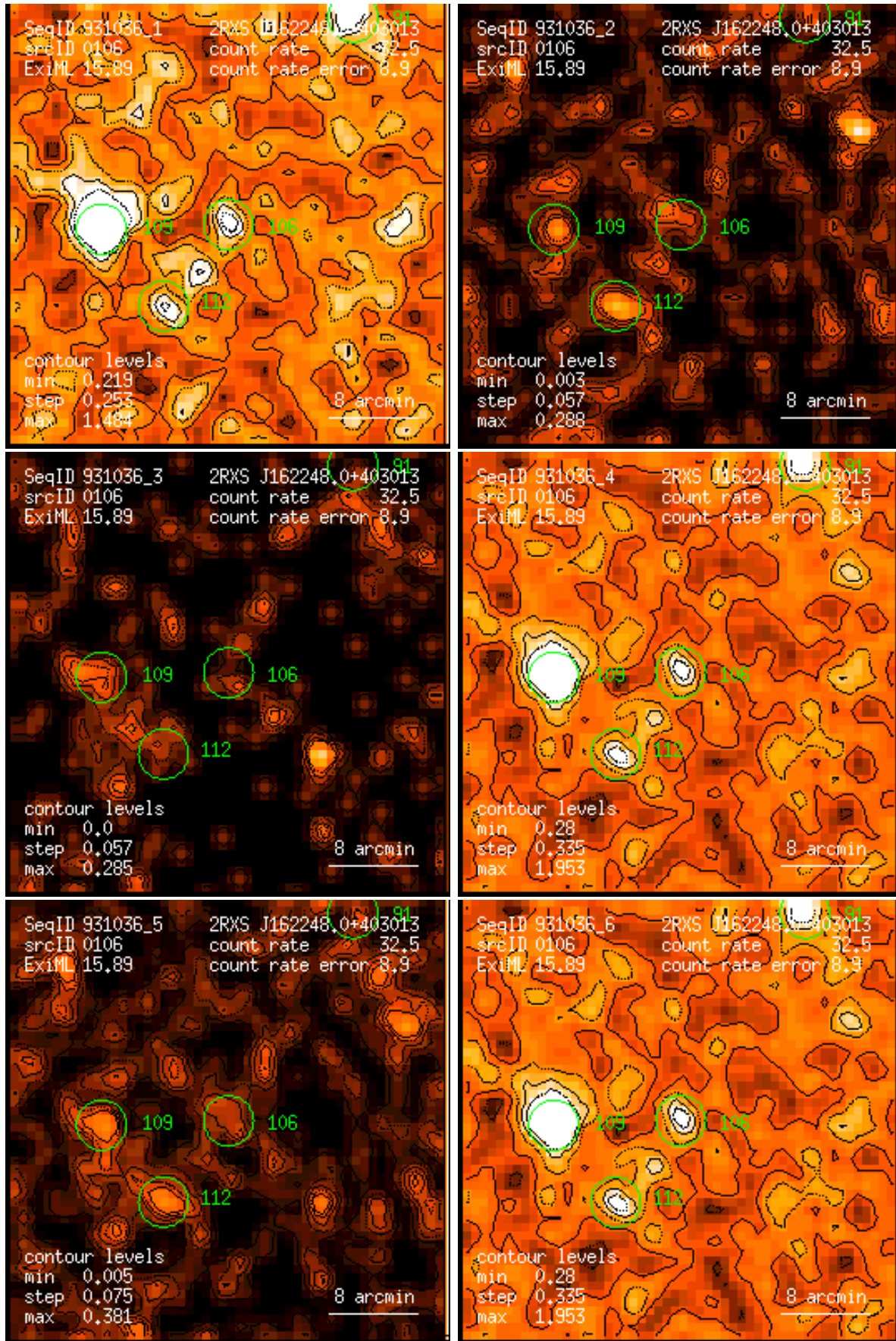
Figure 106: RASS 931036: detection 0106: band rate images, Gaussian filter: (1) PSPC channels 11 – 41, (2) 52 – 90, (3) 91 – 201, (4) 11 – 235, (5) 52 – 201, (6) 11 – 201. Broad band rates in counts/ks. Band rate contour levels in counts/ks/arcmin 2 .
