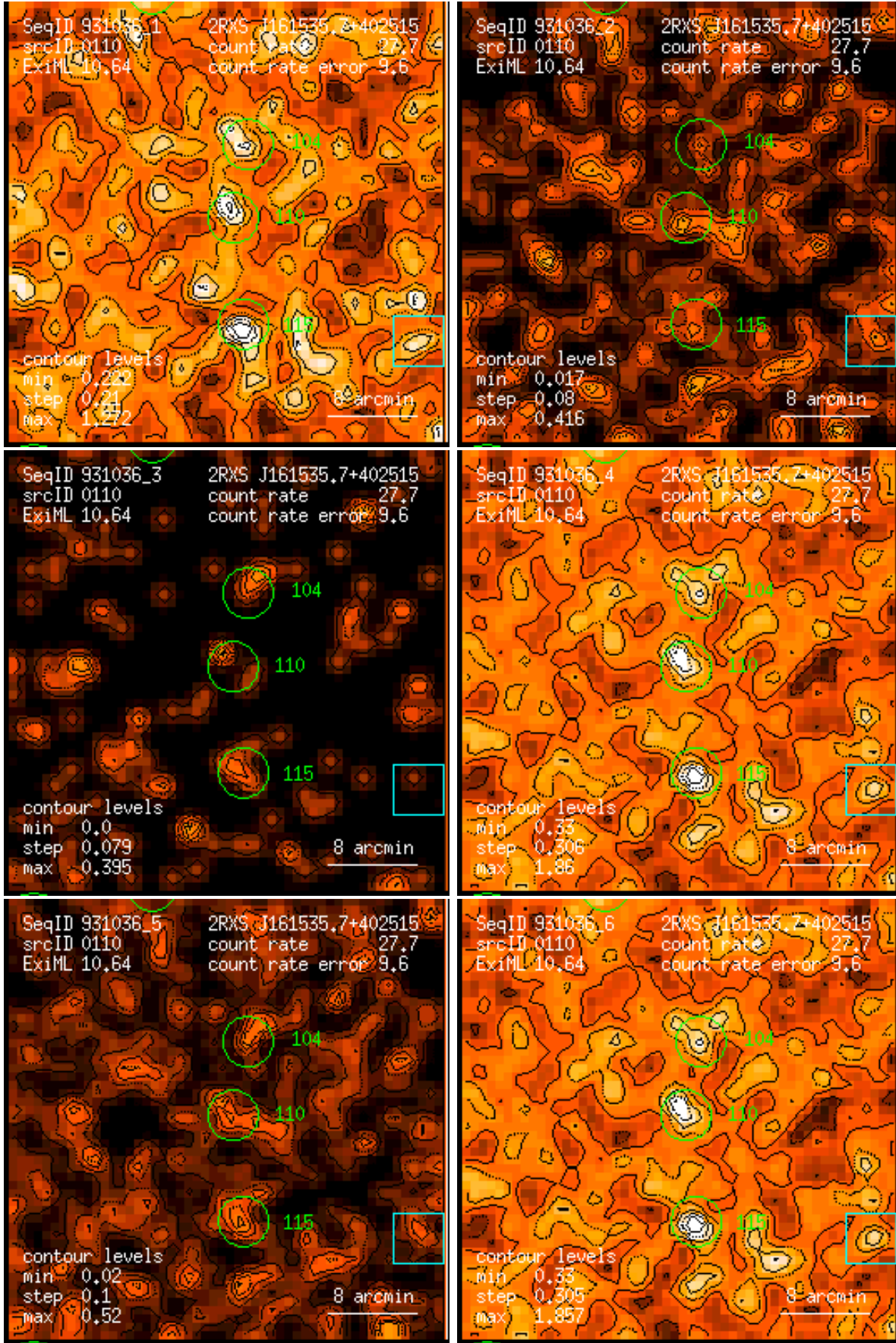
Figure 110: RASS 931036: detection 0110: band rate images, Gaussian filter: (1) PSPC channels 11 – 41, (2) 52 – 90, (3) 91 – 201, (4) 11 – 235, (5) 52 – 201, (6) 11 – 201. Broad band rates in counts/ks. Band rate contour levels in counts/ks/arcmin 2 .
