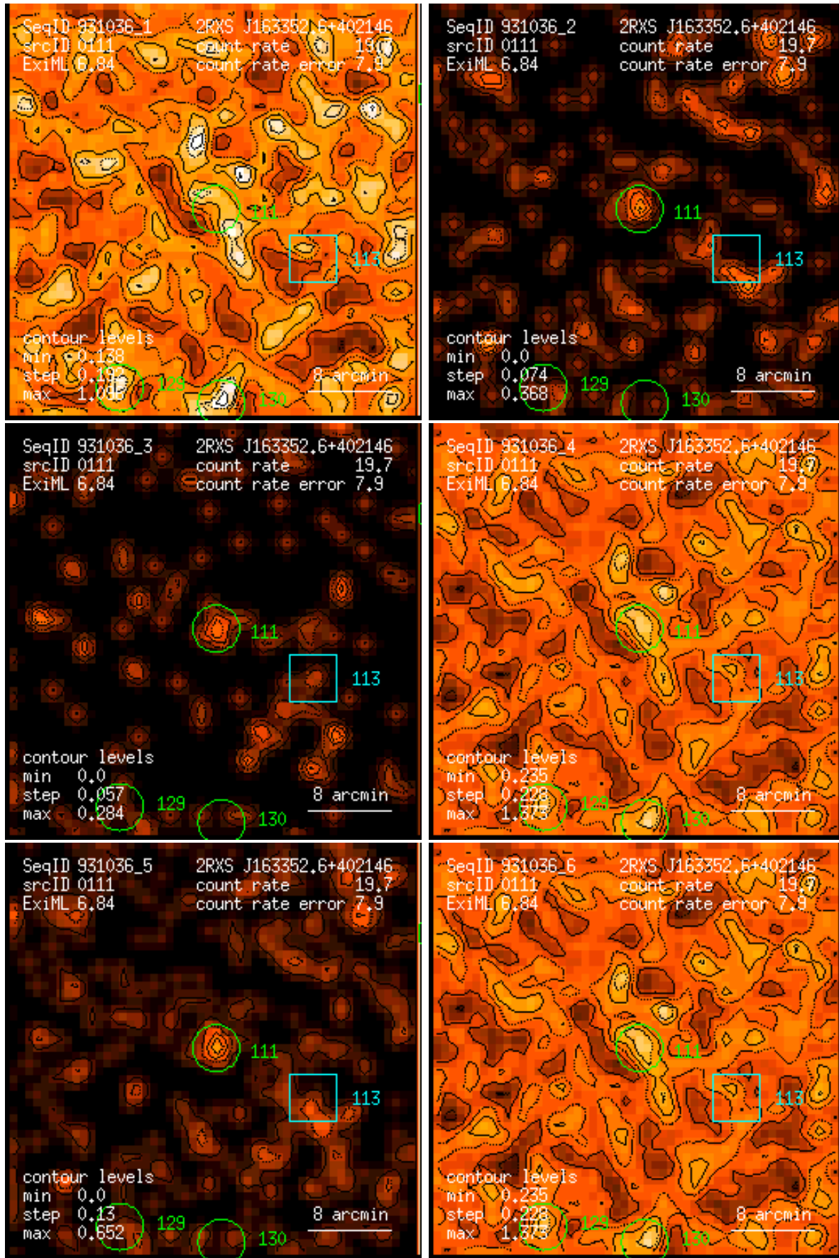
Figure 111: RASS 931036: detection 0111: band rate images, Gaussian filter: (1) PSPC channels 11 – 41, (2) 52 – 90, (3) 91 – 201, (4) 11 – 235, (5) 52 – 201, (6) 11 – 201. Broad band rates in counts/ks. Band rate contour levels in counts/ks/arcmin 2 .
