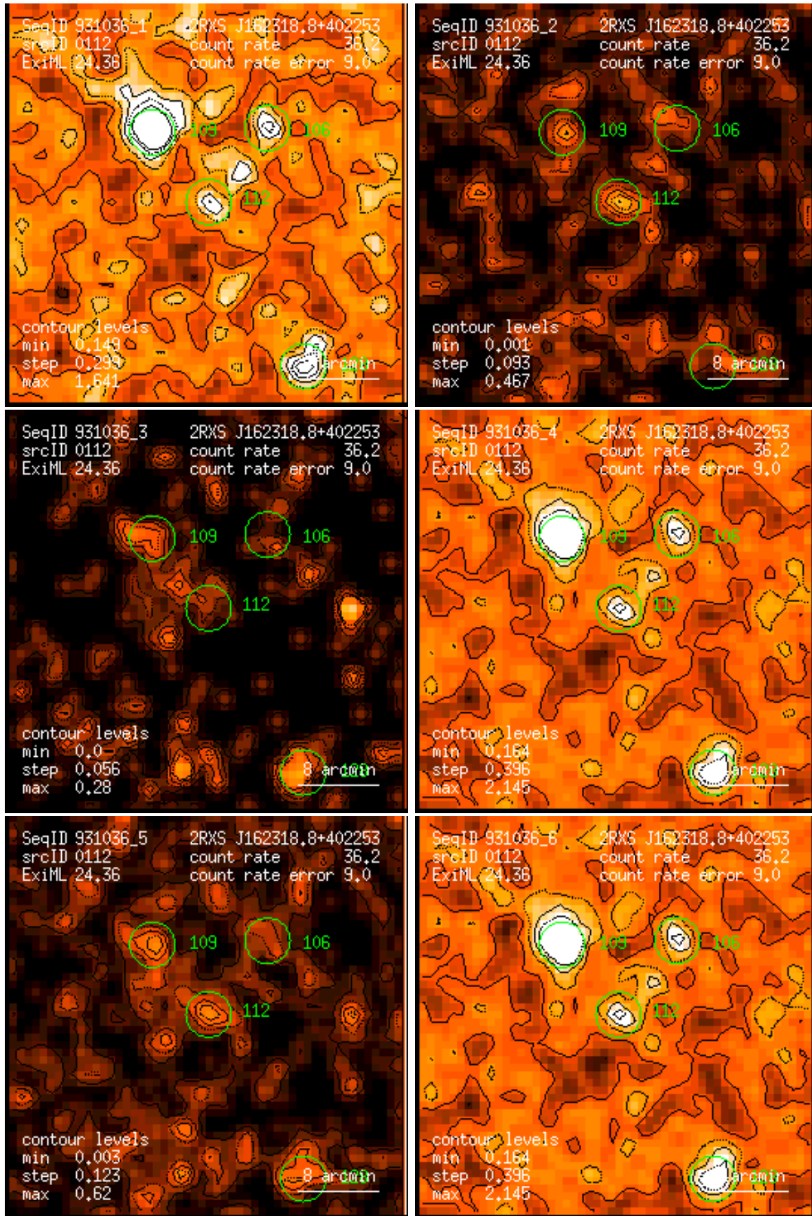
Figure 112: RASS 931036: detection 0112: band rate images, Gaussian filter: (1) PSPC channels 11 – 41, (2) 52 – 90, (3) 91 – 201, (4) 11 – 235, (5) 52 – 201, (6) 11 – 201. Broad band rates in counts/ks. Band rate contour levels in counts/ks/arcmin 2 .
