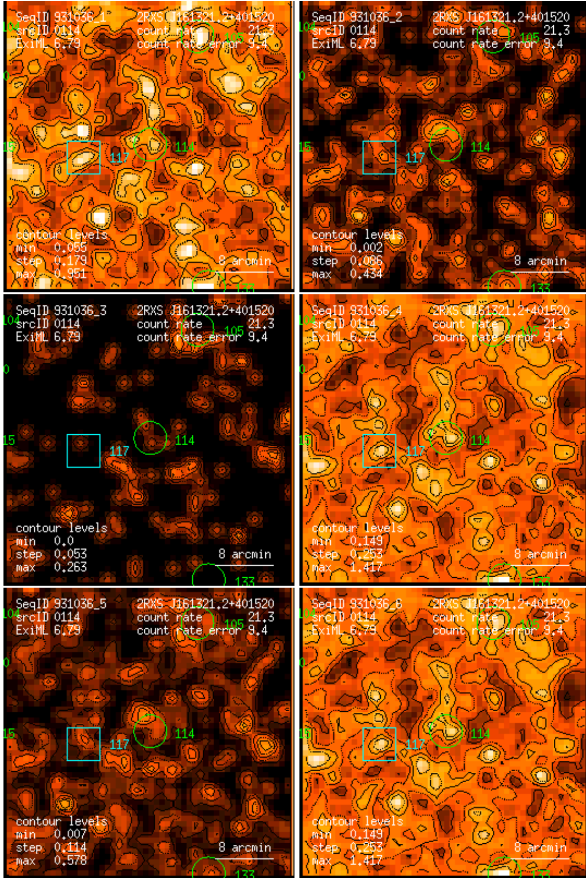
Figure 114: RASS 931036: detection 0114: band rate images, Gaussian filter: (1) PSPC channels 11 – 41, (2) 52 – 90, (3) 91 – 201, (4) 11 – 235, (5) 52 – 201, (6) 11 – 201. Broad band rates in counts/ks. Band rate contour levels in counts/ks/arcmin 2 .
