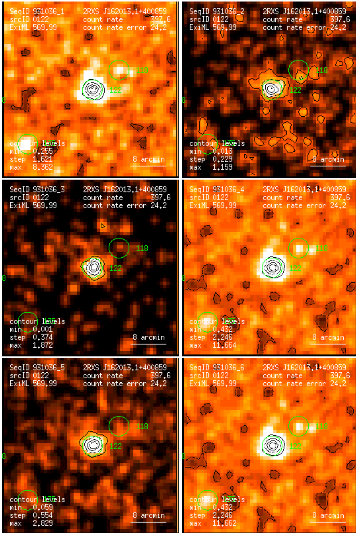
Figure 122: RASS 931036: detection 0122: band rate images, Gaussian filter: (1) PSPC channels 11 – 41, (2) 52 – 90, (3) 91 – 201, (4) 11 – 235, (5) 52 – 201, (6) 11 – 201. Broad band rates in counts/ks. Band rate contour levels in counts/ks/arcmin 2 .
