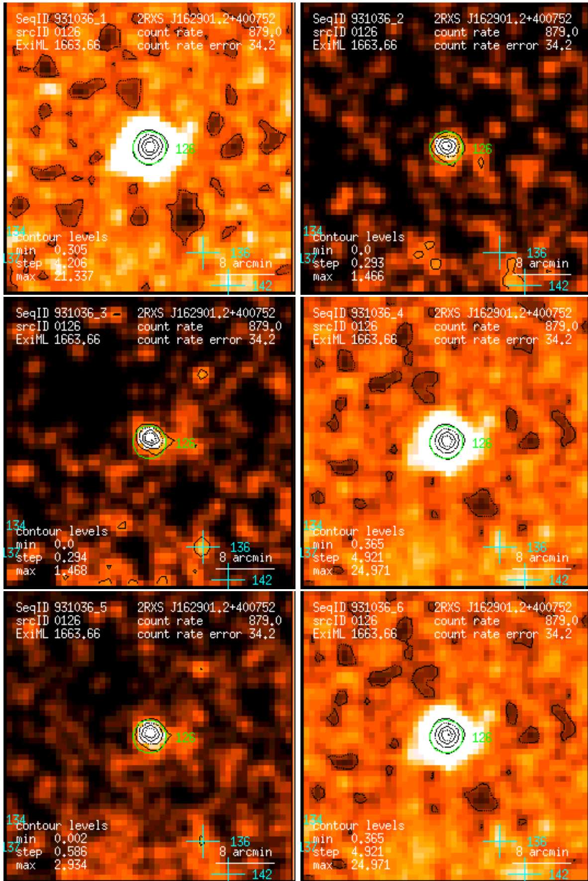
Figure 126: RASS 931036: detection 0126: band rate images, Gaussian filter: (1) PSPC channels 11 – 41, (2) 52 – 90, (3) 91 – 201, (4) 11 – 235, (5) 52 – 201, (6) 11 – 201. Broad band rates in counts/ks. Band rate contour levels in counts/ks/arcmin 2 .
