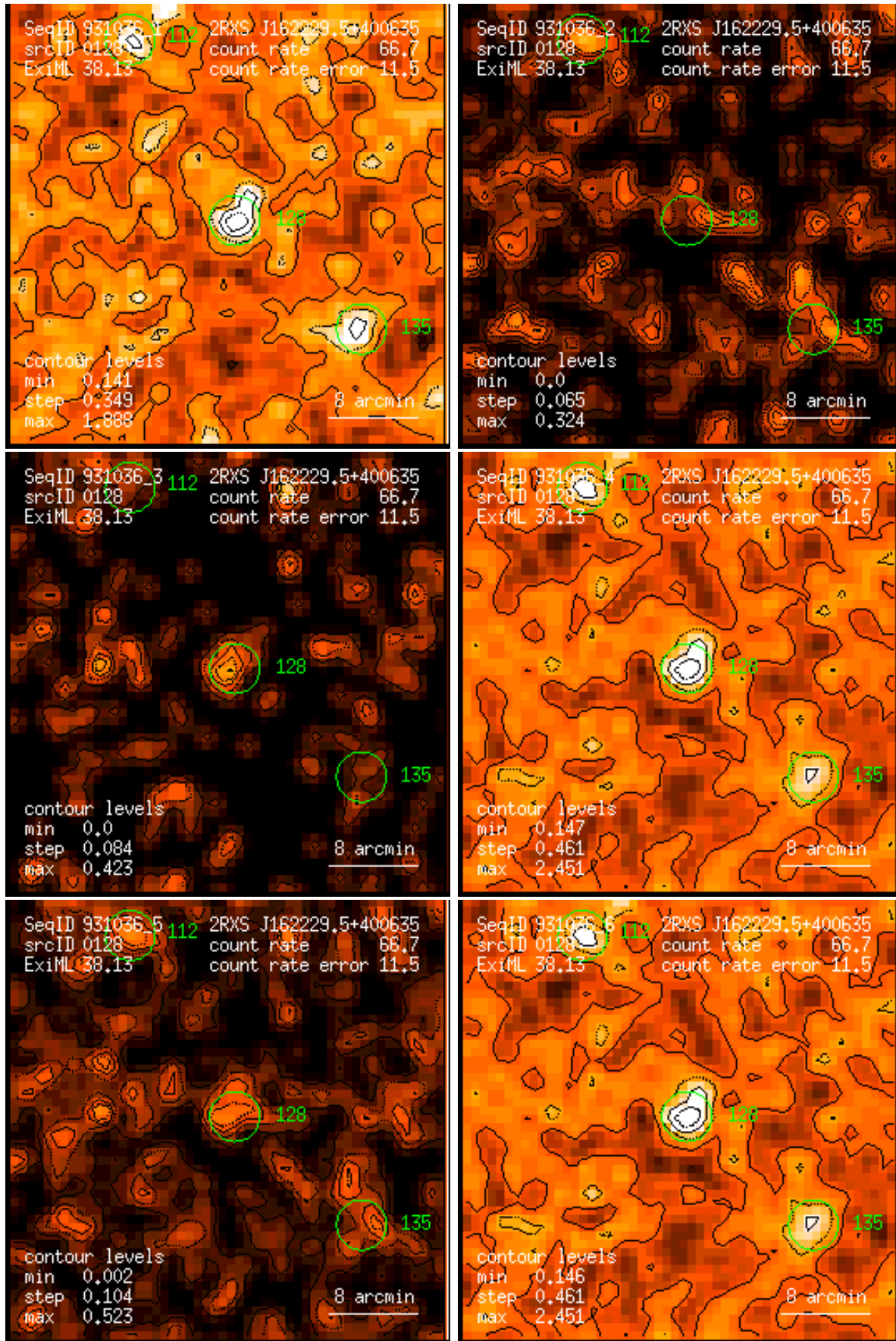
Figure 128: RASS 931036: detection 0128: band rate images, Gaussian filter: (1) PSPC channels 11 – 41, (2) 52 – 90, (3) 91 – 201, (4) 11 – 235, (5) 52 – 201, (6) 11 – 201. Broad band rates in counts/ks. Band rate contour levels in counts/ks/arcmin 2 .
