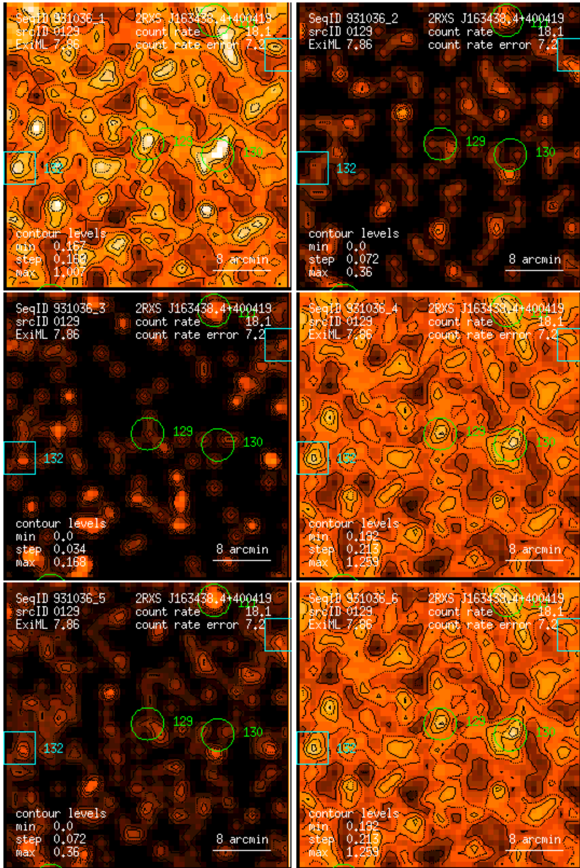
Figure 129: RASS 931036: detection 0129: band rate images, Gaussian filter: (1) PSPC channels 11 – 41, (2) 52 – 90, (3) 91 – 201, (4) 11 – 235, (5) 52 – 201, (6) 11 – 201. Broad band rates in counts/ks. Band rate contour levels in counts/ks/arcmin 2 .
