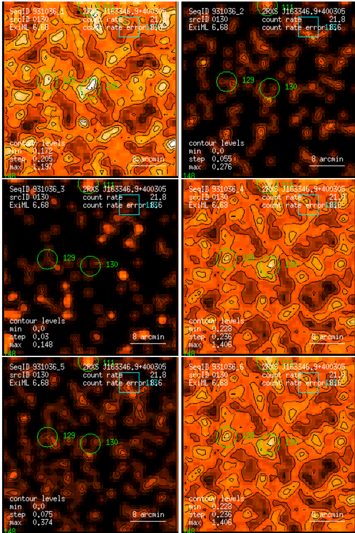
Figure 130: RASS 931036: detection 0130: band rate images, Gaussian filter: (1) PSPC channels 11 – 41, (2) 52 – 90, (3) 91 – 201, (4) 11 – 235, (5) 52 – 201, (6) 11 – 201. Broad band rates in counts/ks. Band rate contour levels in counts/ks/arcmin 2 .
