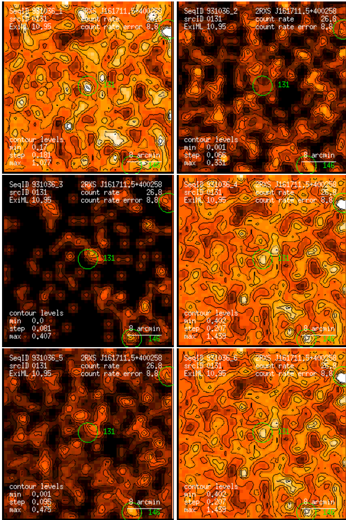
Figure 131: RASS 931036: detection 0131: band rate images, Gaussian filter: (1) PSPC channels 11 – 41, (2) 52 – 90, (3) 91 – 201, (4) 11 – 235, (5) 52 – 201, (6) 11 – 201. Broad band rates in counts/ks. Band rate contour levels in counts/ks/arcmin 2 .
