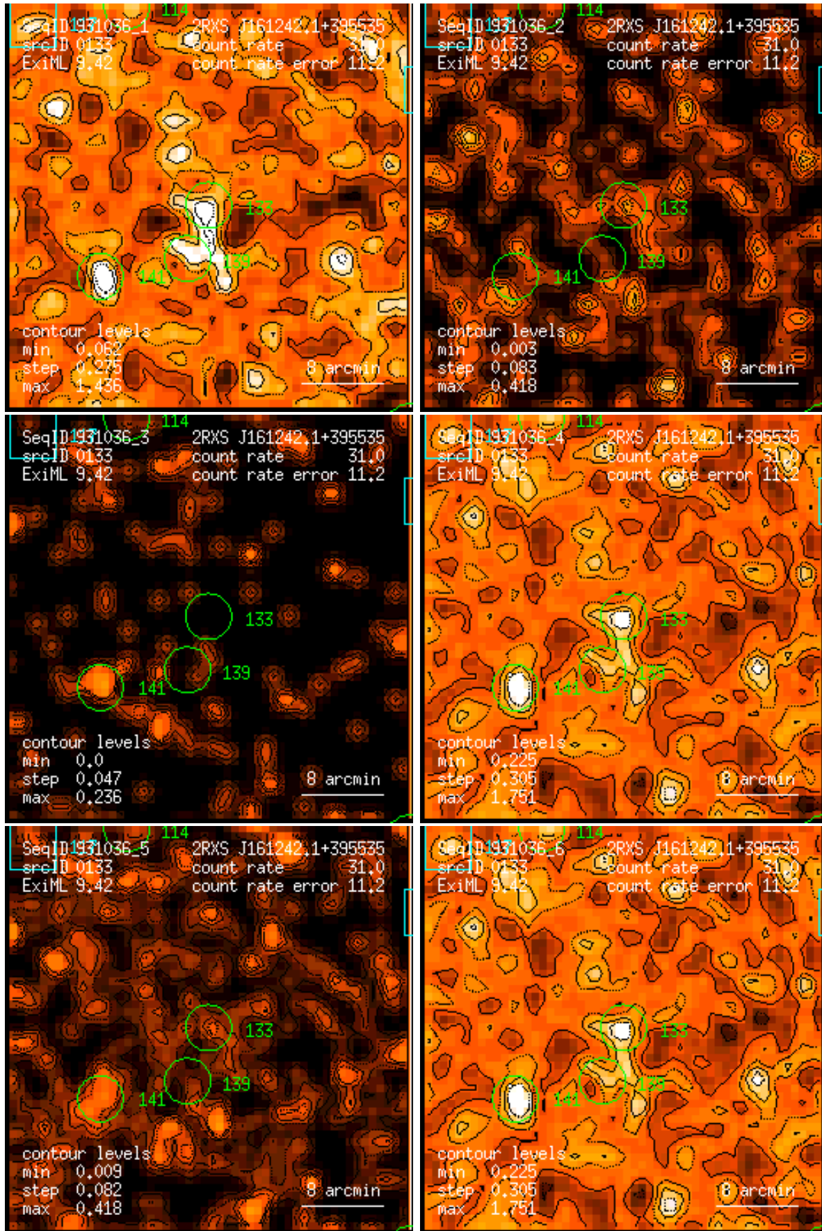
Figure 133: RASS 931036: detection 0133: band rate images, Gaussian filter: (1) PSPC channels 11 – 41, (2) 52 – 90, (3) 91 – 201, (4) 11 – 235, (5) 52 – 201, (6) 11 – 201. Broad band rates in counts/ks. Band rate contour levels in counts/ks/arcmin 2 .
