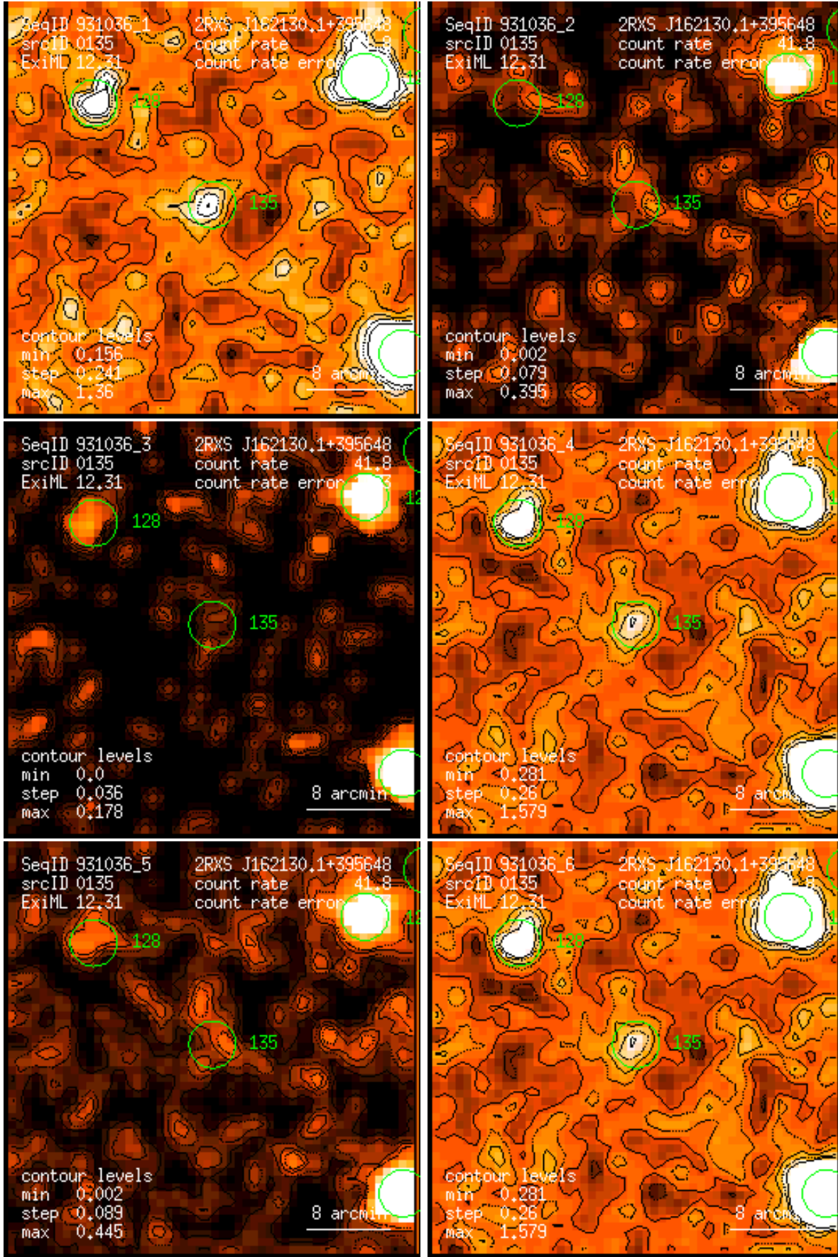
Figure 135: RASS 931036: detection 0135: band rate images, Gaussian filter: (1) PSPC channels 11 – 41, (2) 52 – 90, (3) 91 – 201, (4) 11 – 235, (5) 52 – 201, (6) 11 – 201. Broad band rates in counts/ks. Band rate contour levels in counts/ks/arcmin 2 .
