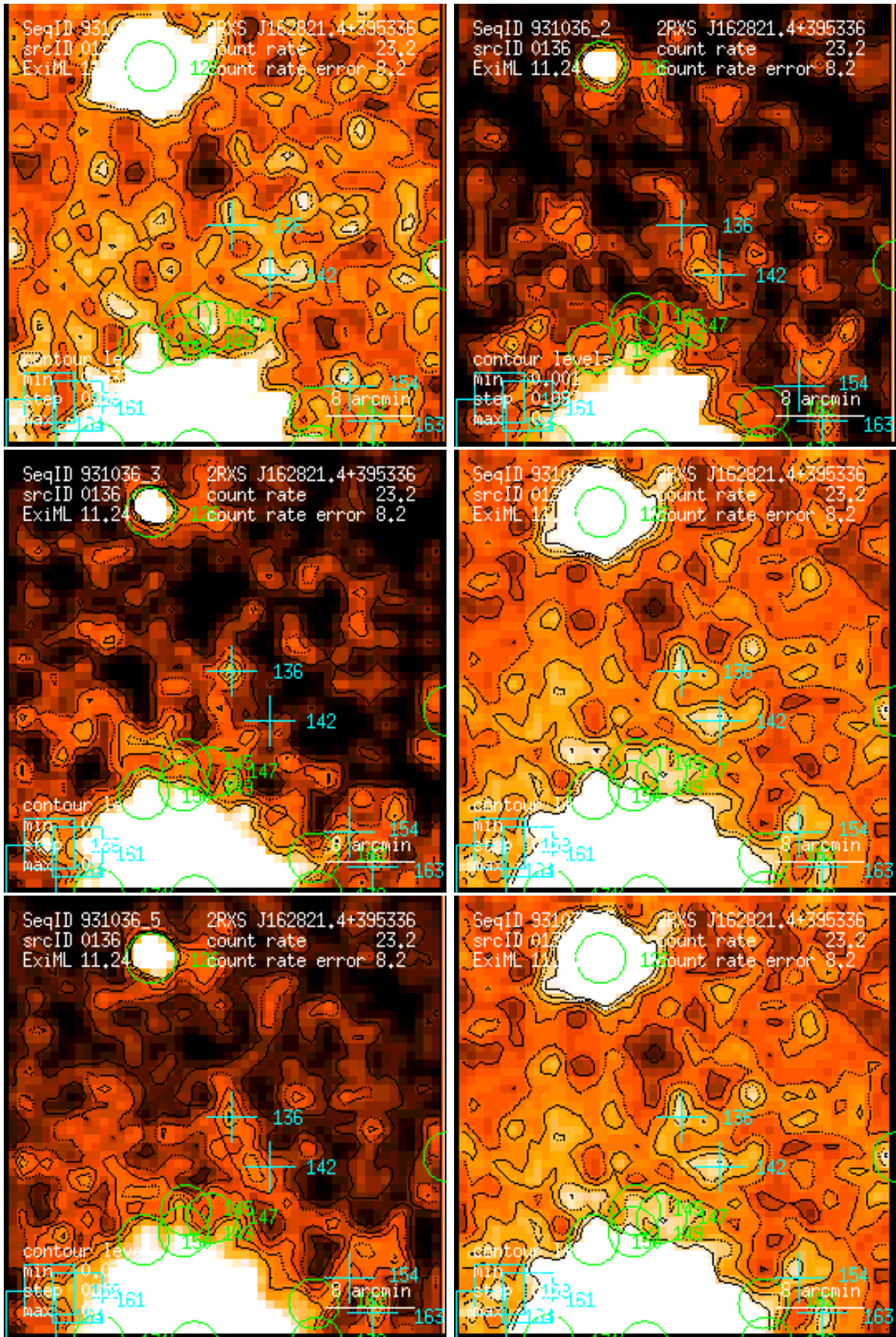
Figure 136: RASS 931036: detection 0136: band rate images, Gaussian filter: (1) PSPC channels 11 – 41, (2) 52 – 90, (3) 91 – 201, (4) 11 – 235, (5) 52 – 201, (6) 11 – 201. Broad band rates in counts/ks. Band rate contour levels in counts/ks/arcmin 2 .
