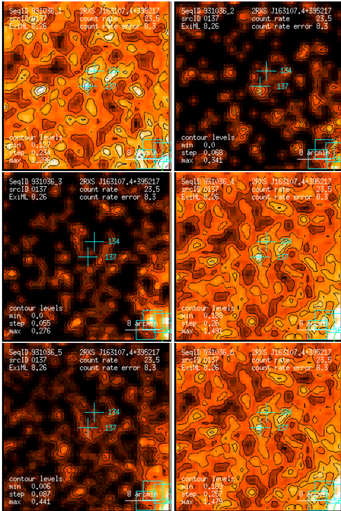
Figure 137: RASS 931036: detection 0137: band rate images, Gaussian filter: (1) PSPC channels 11 – 41, (2) 52 – 90, (3) 91 – 201, (4) 11 – 235, (5) 52 – 201, (6) 11 – 201. Broad band rates in counts/ks. Band rate contour levels in counts/ks/arcmin 2 .
