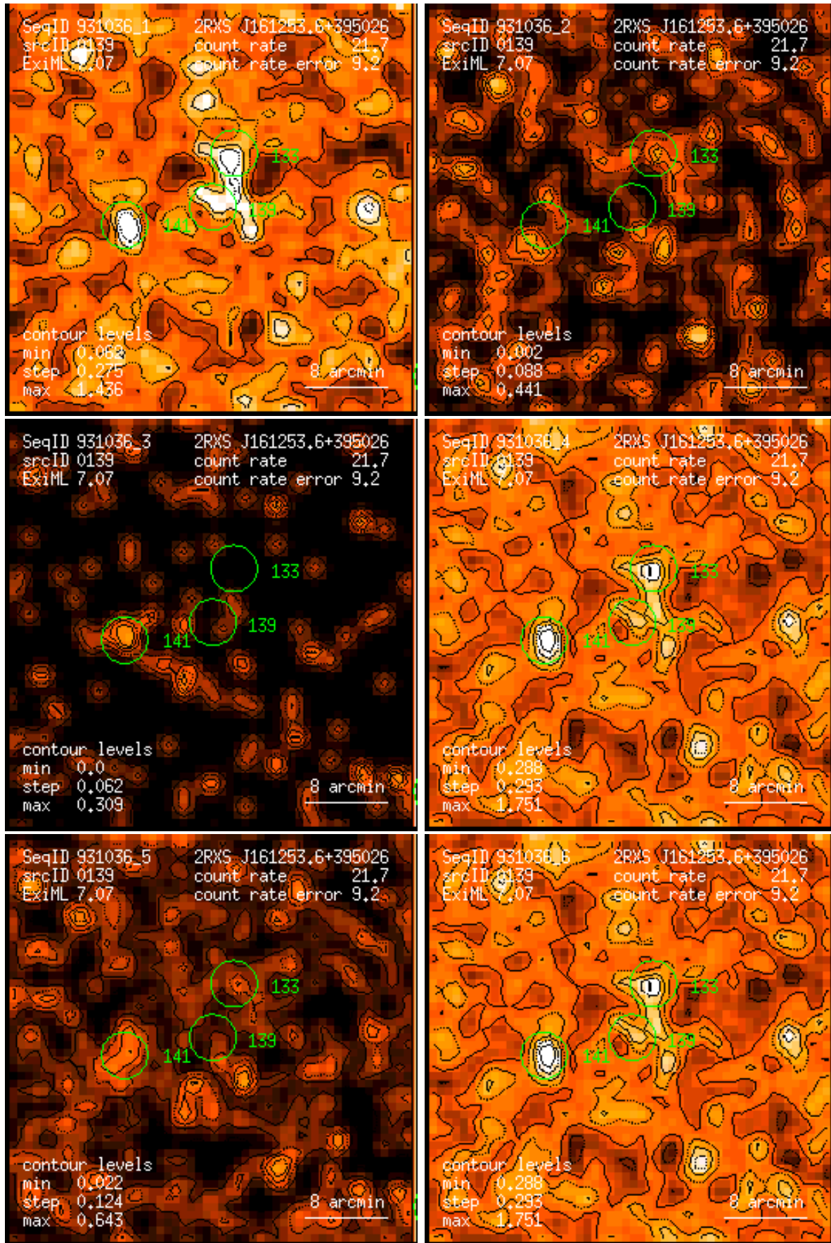
Figure 139: RASS 931036: detection 0139: band rate images, Gaussian filter: (1) PSPC channels 11 – 41, (2) 52 – 90, (3) 91 – 201, (4) 11 – 235, (5) 52 – 201, (6) 11 – 201. Broad band rates in counts/ks. Band rate contour levels in counts/ks/arcmin 2 .
