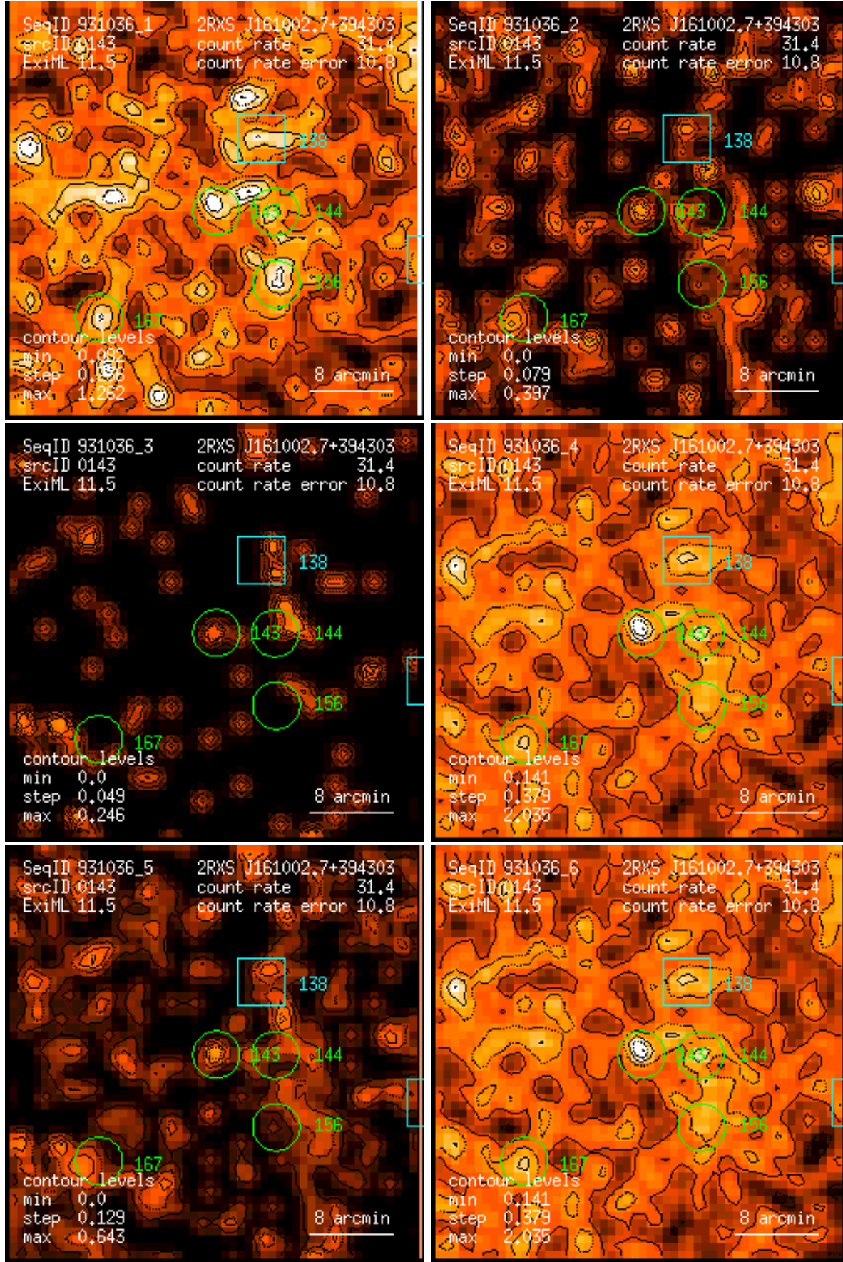
Figure 143: RASS 931036: detection 0143: band rate images, Gaussian filter: (1) PSPC channels 11 – 41, (2) 52 – 90, (3) 91 – 201, (4) 11 – 235, (5) 52 – 201, (6) 11 – 201. Broad band rates in counts/ks. Band rate contour levels in counts/ks/arcmin 2 .
