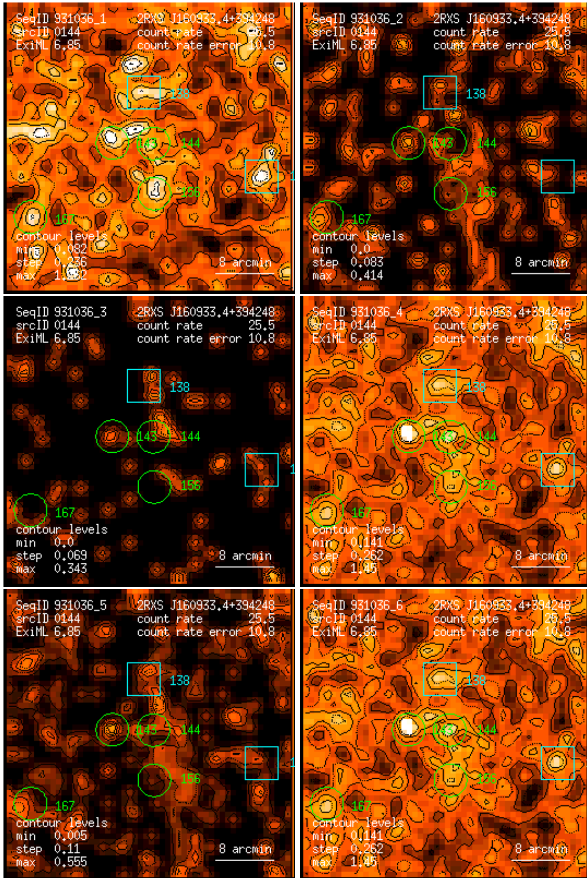
Figure 144: RASS 931036: detection 0144: band rate images, Gaussian filter: (1) PSPC channels 11 – 41, (2) 52 – 90, (3) 91 – 201, (4) 11 – 235, (5) 52 – 201, (6) 11 – 201. Broad band rates in counts/ks. Band rate contour levels in counts/ks/arcmin 2 .
