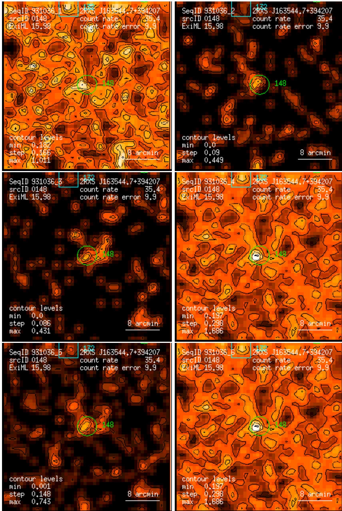
Figure 148: RASS 931036: detection 0148: band rate images, Gaussian filter: (1) PSPC channels 11 – 41, (2) 52 – 90, (3) 91 – 201, (4) 11 – 235, (5) 52 – 201, (6) 11 – 201. Broad band rates in counts/ks. Band rate contour levels in counts/ks/arcmin 2 .
