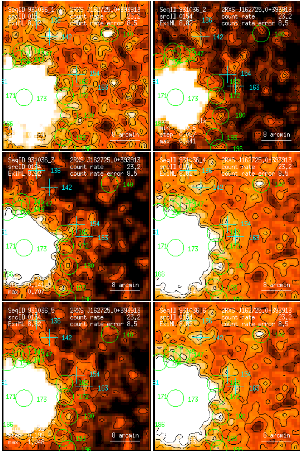
Figure 154: RASS 931036: detection 0154: band rate images, Gaussian filter: (1) PSPC channels 11 – 41, (2) 52 – 90, (3) 91 – 201, (4) 11 – 235, (5) 52 – 201, (6) 11 – 201. Broad band rates in counts/ks. Band rate contour levels in counts/ks/arcmin 2 .
