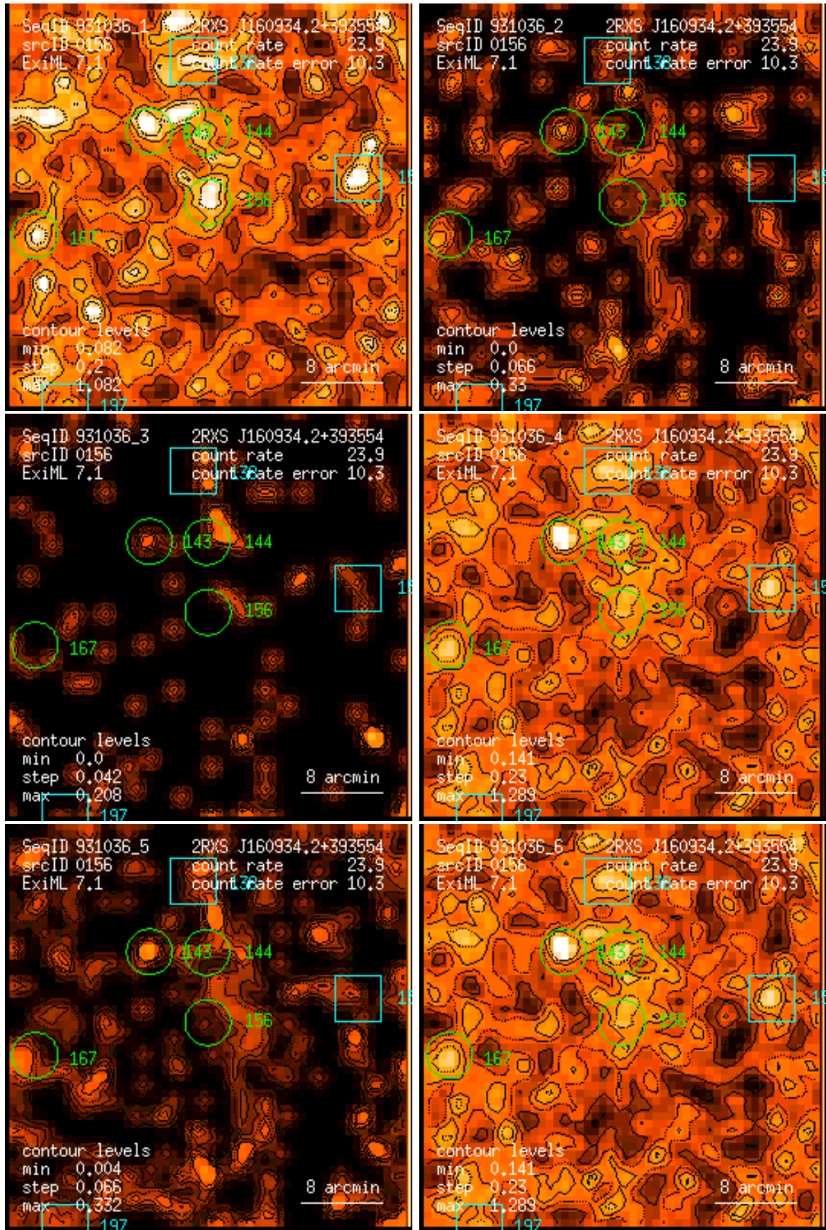
Figure 156: RASS 931036: detection 0156: band rate images, Gaussian filter: (1) PSPC channels 11 – 41, (2) 52 – 90, (3) 91 – 201, (4) 11 – 235, (5) 52 – 201, (6) 11 – 201. Broad band rates in counts/ks. Band rate contour levels in counts/ks/arcmin 2 .
