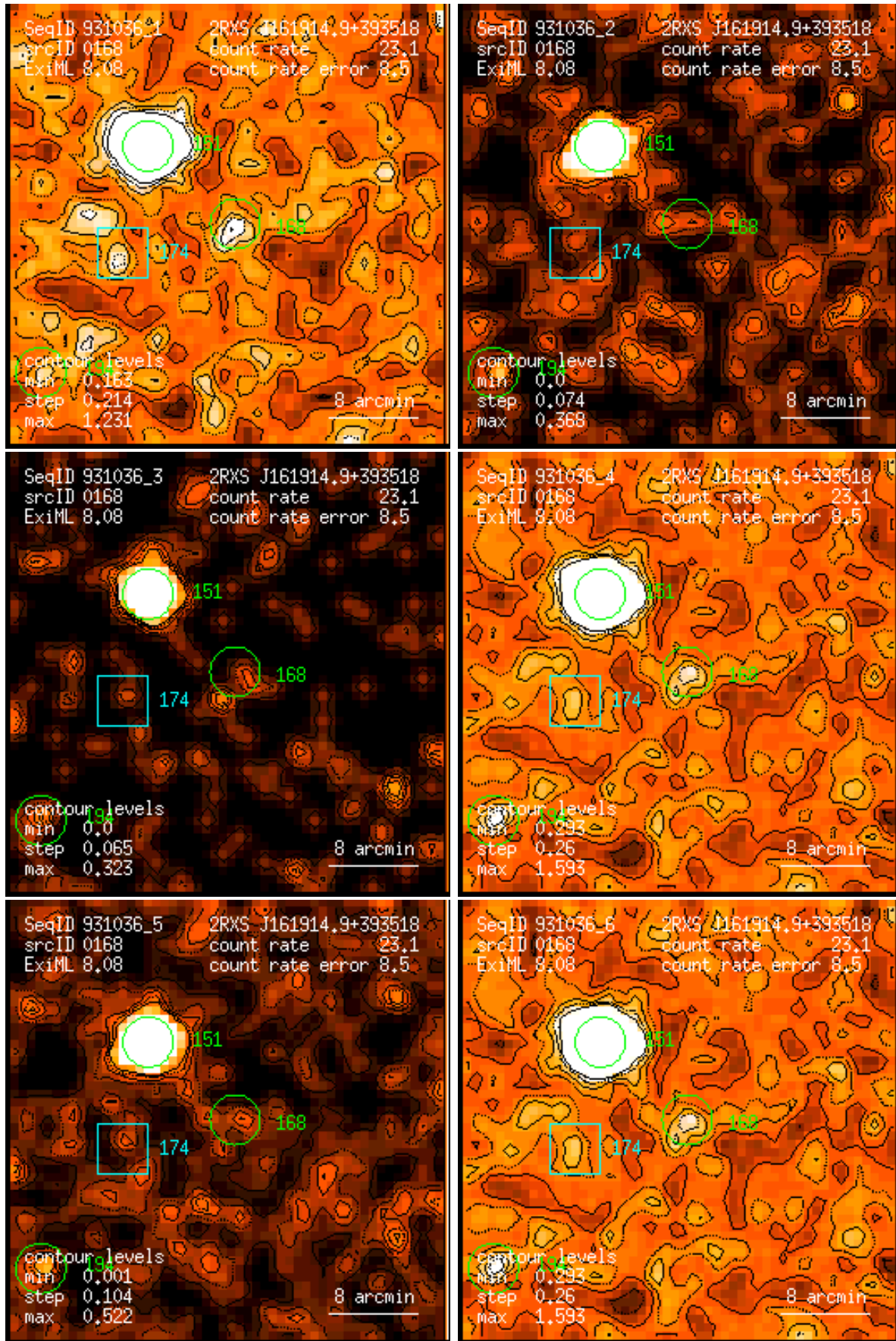
Figure 168: RASS 931036: detection 0168: band rate images, Gaussian filter: (1) PSPC channels 11 – 41, (2) 52 – 90, (3) 91 – 201, (4) 11 – 235, (5) 52 – 201, (6) 11 – 201. Broad band rates in counts/ks. Band rate contour levels in counts/ks/arcmin 2 .
